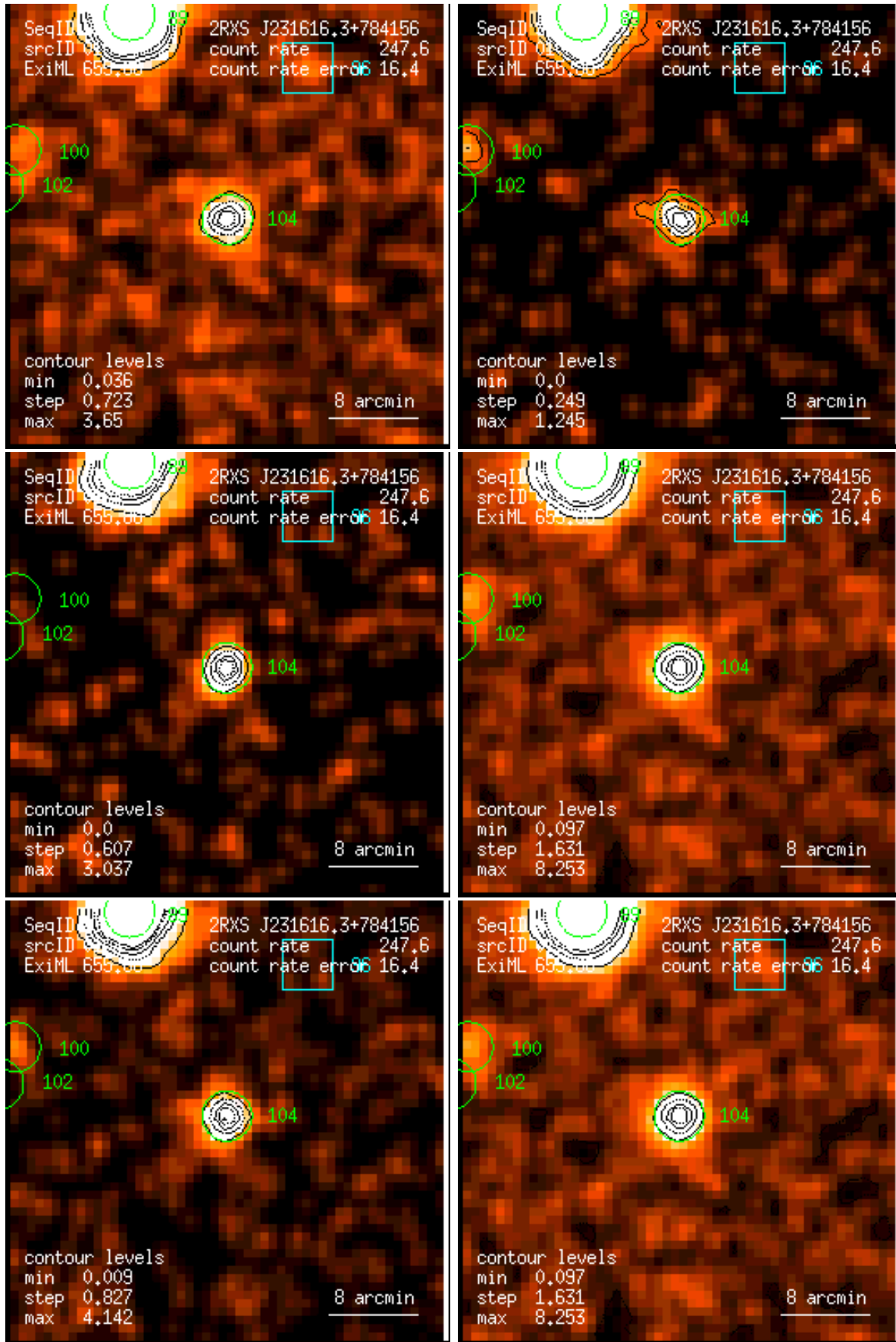
Figure 104: RASS 930316: detection 0104: band rate images, Gaussian filter: (1) PSPC channels 11 – 41, (2) 52 – 90, (3) 91 – 201, (4) 11 – 235, (5) 52 – 201, (6) 11 – 201. Broad band rates in counts/ks. Band rate contour levels in counts/ks/arcmin 2 .
