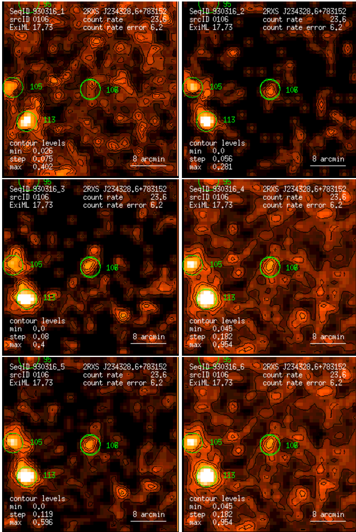
Figure 106: RASS 930316: detection 0106: band rate images, Gaussian filter: (1) PSPC channels 11 – 41, (2) 52 – 90, (3) 91 – 201, (4) 11 – 235, (5) 52 – 201, (6) 11 – 201. Broad band rates in counts/ks. Band rate contour levels in counts/ks/arcmin 2 .
