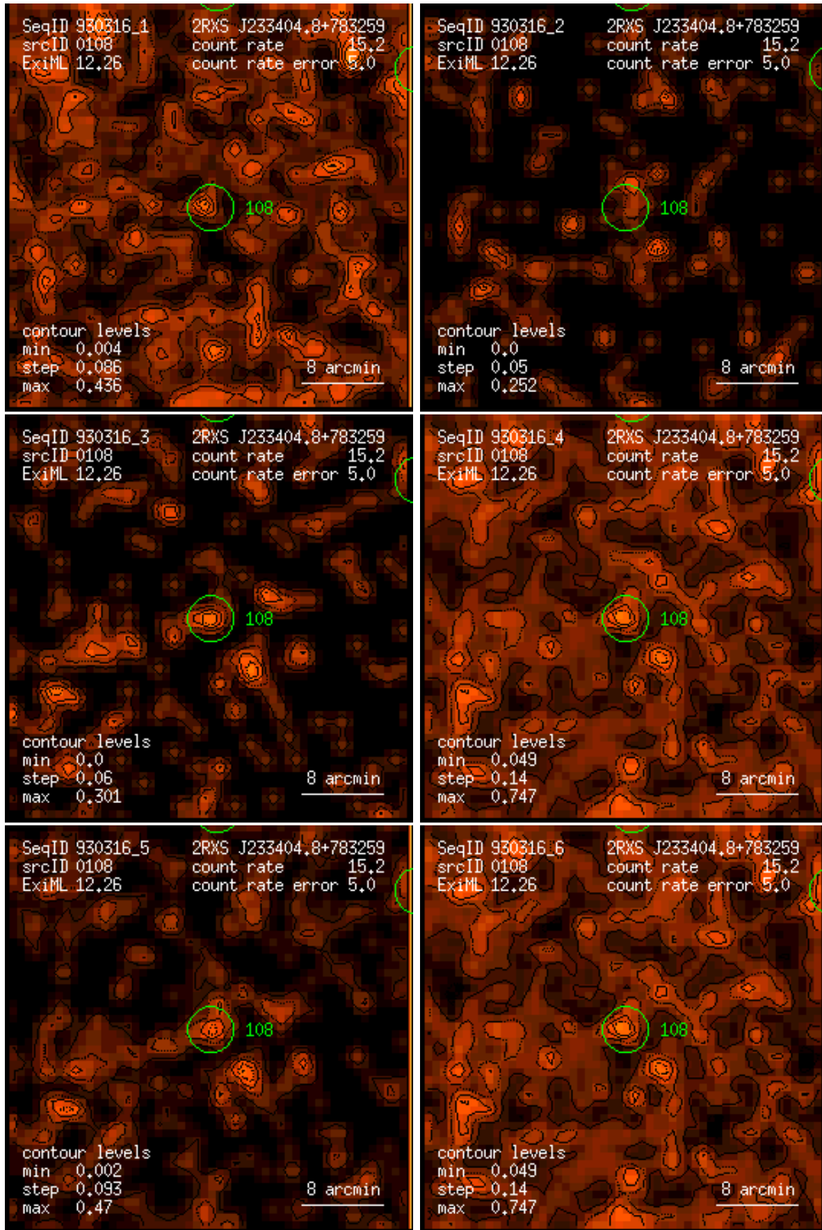
Figure 108: RASS 930316: detection 0108: band rate images, Gaussian filter: (1) PSPC channels 11 – 41, (2) 52 – 90, (3) 91 – 201, (4) 11 – 235, (5) 52 – 201, (6) 11 – 201. Broad band rates in counts/ks. Band rate contour levels in counts/ks/arcmin 2 .
