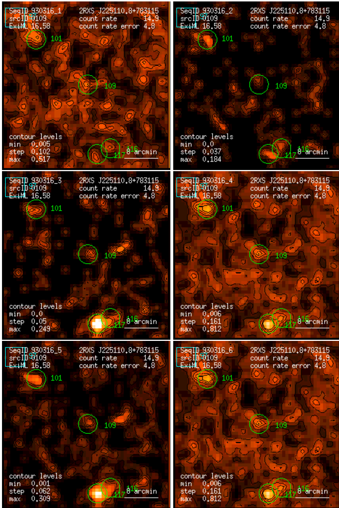
Figure 109: RASS 930316: detection 0109: band rate images, Gaussian filter: (1) PSPC channels 11 – 41, (2) 52 – 90, (3) 91 – 201, (4) 11 – 235, (5) 52 – 201, (6) 11 – 201. Broad band rates in counts/ks. Band rate contour levels in counts/ks/arcmin 2 .
