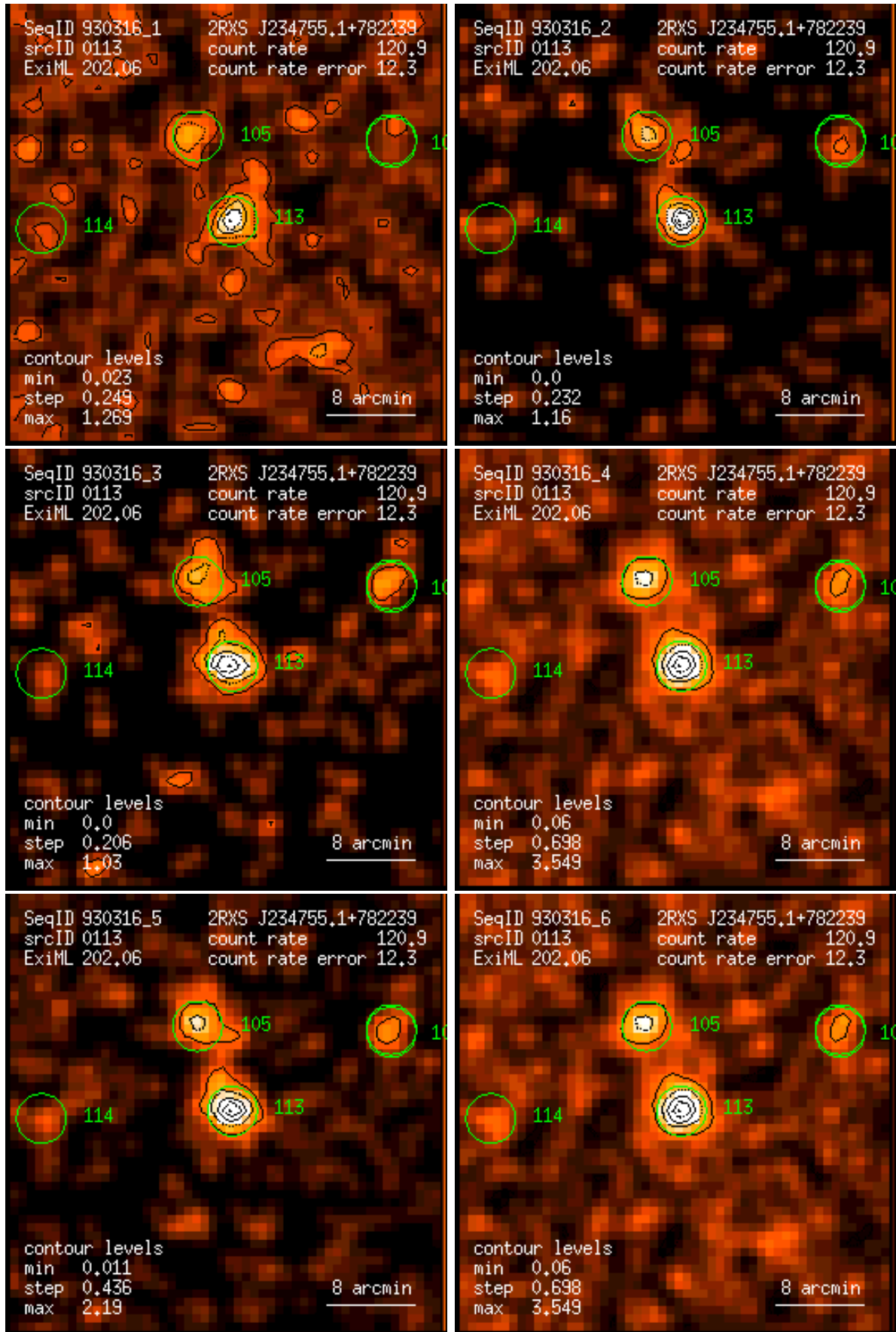
Figure 113: RASS 930316: detection 0113: band rate images, Gaussian filter: (1) PSPC channels 11 – 41, (2) 52 – 90, (3) 91 – 201, (4) 11 – 235, (5) 52 – 201, (6) 11 – 201. Broad band rates in counts/ks. Band rate contour levels in counts/ks/arcmin 2 .
