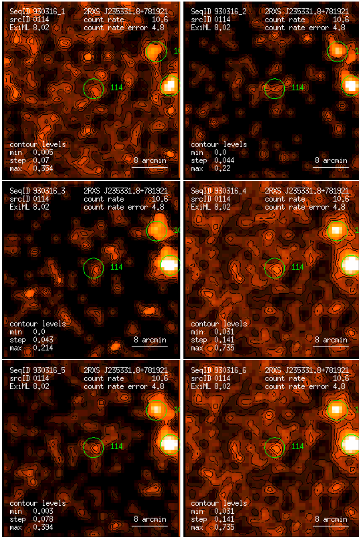
Figure 114: RASS 930316: detection 0114: band rate images, Gaussian filter: (1) PSPC channels 11 – 41, (2) 52 – 90, (3) 91 – 201, (4) 11 – 235, (5) 52 – 201, (6) 11 – 201. Broad band rates in counts/ks. Band rate contour levels in counts/ks/arcmin 2 .
