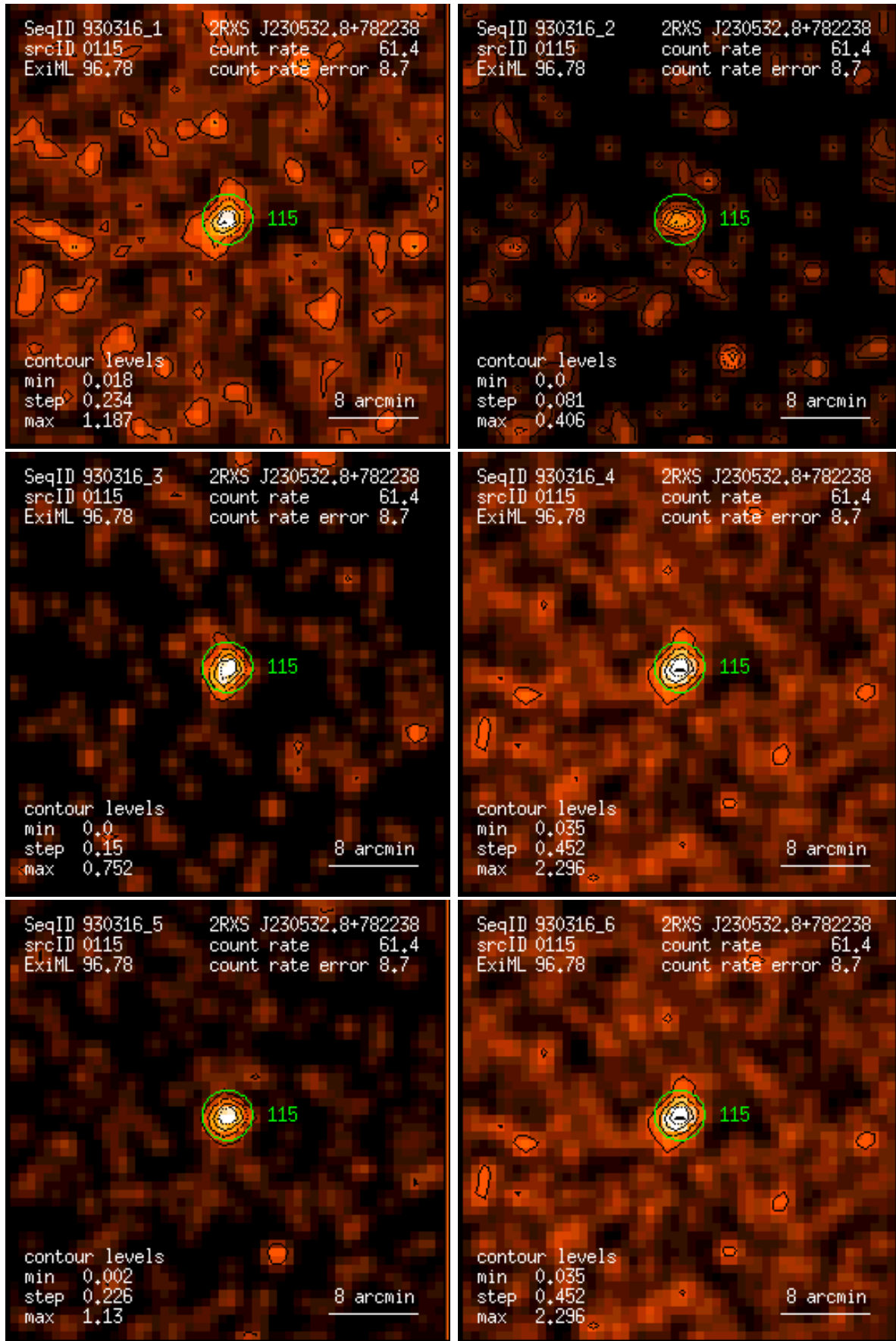
Figure 115: RASS 930316: detection 0115: band rate images, Gaussian filter: (1) PSPC channels 11 – 41, (2) 52 – 90, (3) 91 – 201, (4) 11 – 235, (5) 52 – 201, (6) 11 – 201. Broad band rates in counts/ks. Band rate contour levels in counts/ks/arcmin 2 .
