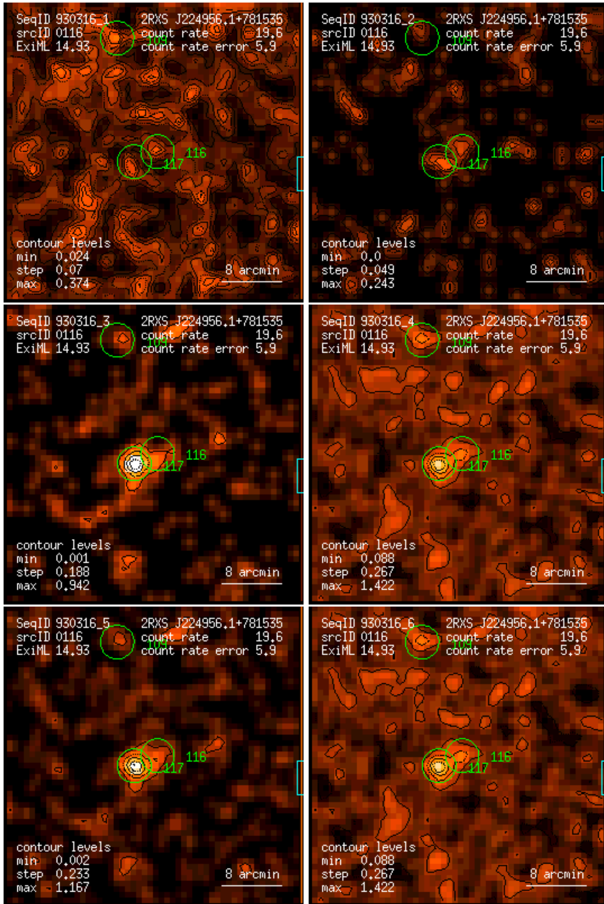
Figure 116: RASS 930316: detection 0116: band rate images, Gaussian filter: (1) PSPC channels 11 – 41, (2) 52 – 90, (3) 91 – 201, (4) 11 – 235, (5) 52 – 201, (6) 11 – 201. Broad band rates in counts/ks. Band rate contour levels in counts/ks/arcmin 2 .
