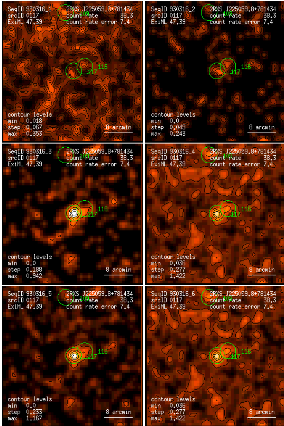
Figure 117: RASS 930316: detection 0117: band rate images, Gaussian filter: (1) PSPC channels 11 – 41, (2) 52 – 90, (3) 91 – 201, (4) 11 – 235, (5) 52 – 201, (6) 11 – 201. Broad band rates in counts/ks. Band rate contour levels in counts/ks/arcmin 2 .
