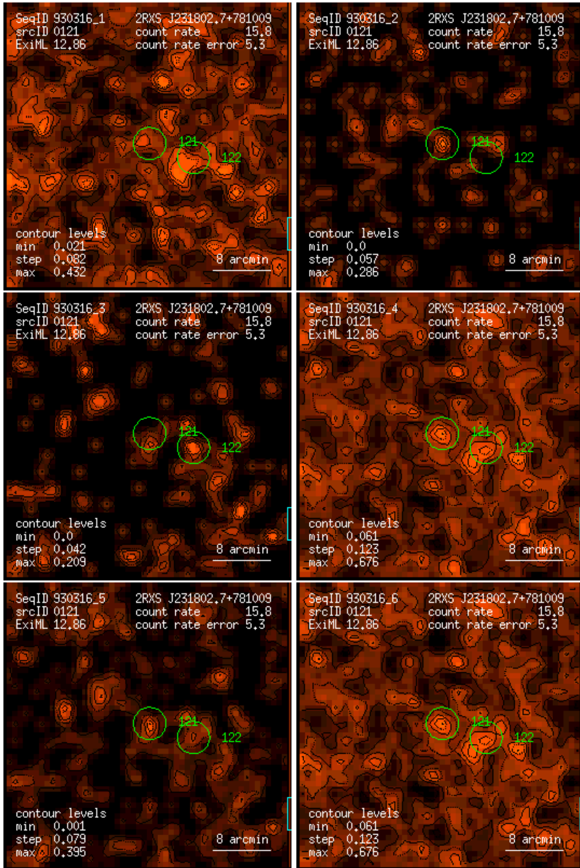
Figure 121: RASS 930316: detection 0121: band rate images, Gaussian filter: (1) PSPC channels 11 – 41, (2) 52 – 90, (3) 91 – 201, (4) 11 – 235, (5) 52 – 201, (6) 11 – 201. Broad band rates in counts/ks. Band rate contour levels in counts/ks/arcmin 2 .
