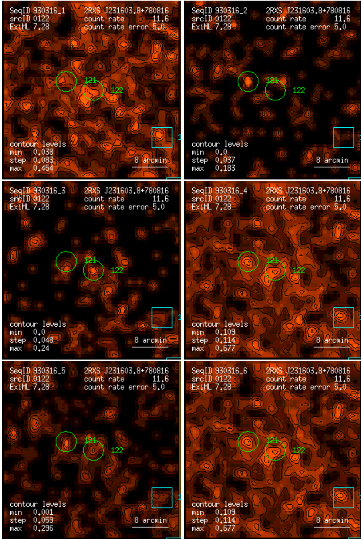
Figure 122: RASS 930316: detection 0122: band rate images, Gaussian filter: (1) PSPC channels 11 – 41, (2) 52 – 90, (3) 91 – 201, (4) 11 – 235, (5) 52 – 201, (6) 11 – 201. Broad band rates in counts/ks. Band rate contour levels in counts/ks/arcmin 2 .
