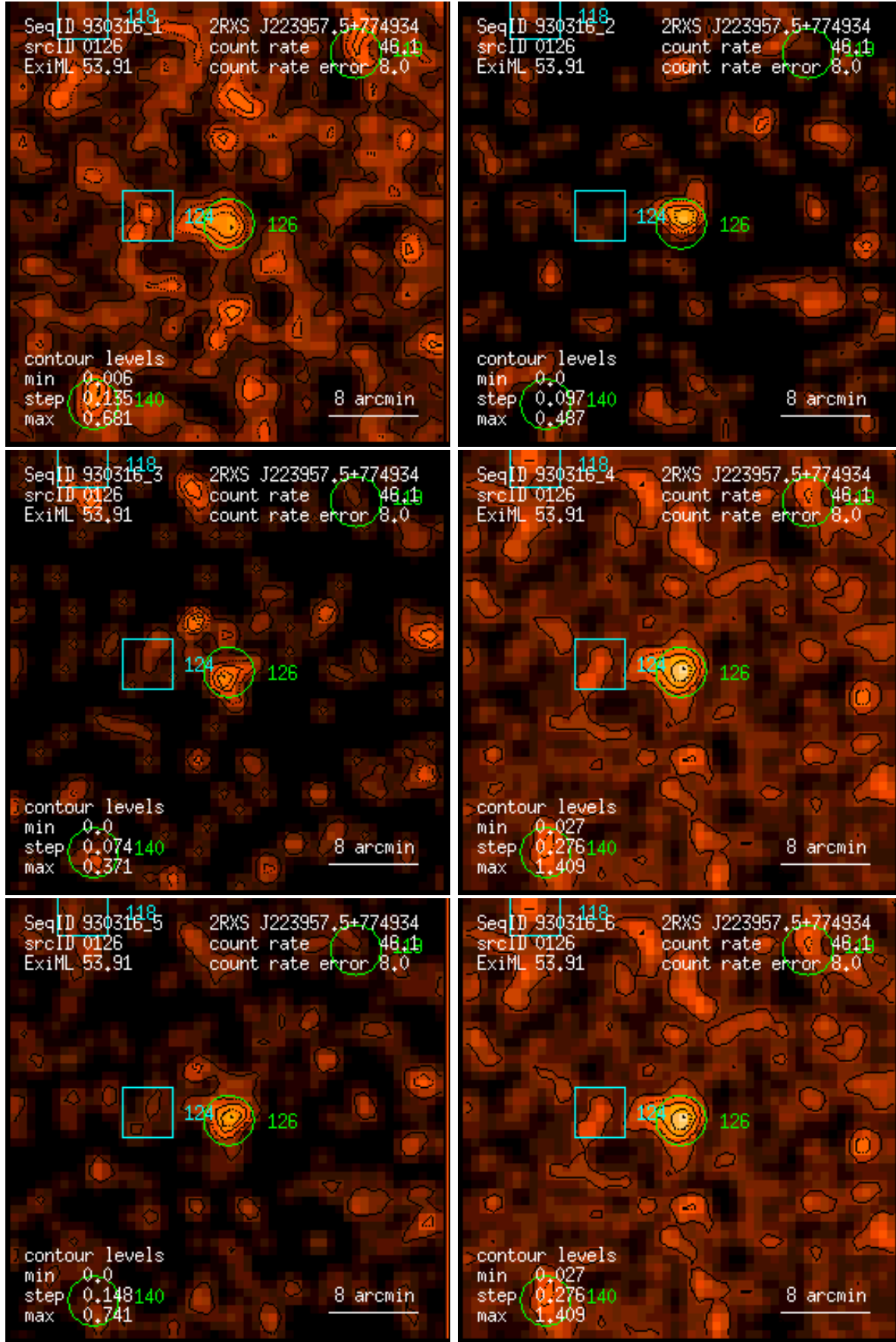
Figure 126: RASS 930316: detection 0126: band rate images, Gaussian filter: (1) PSPC channels 11 – 41, (2) 52 – 90, (3) 91 – 201, (4) 11 – 235, (5) 52 – 201, (6) 11 – 201. Broad band rates in counts/ks. Band rate contour levels in counts/ks/arcmin 2 .
