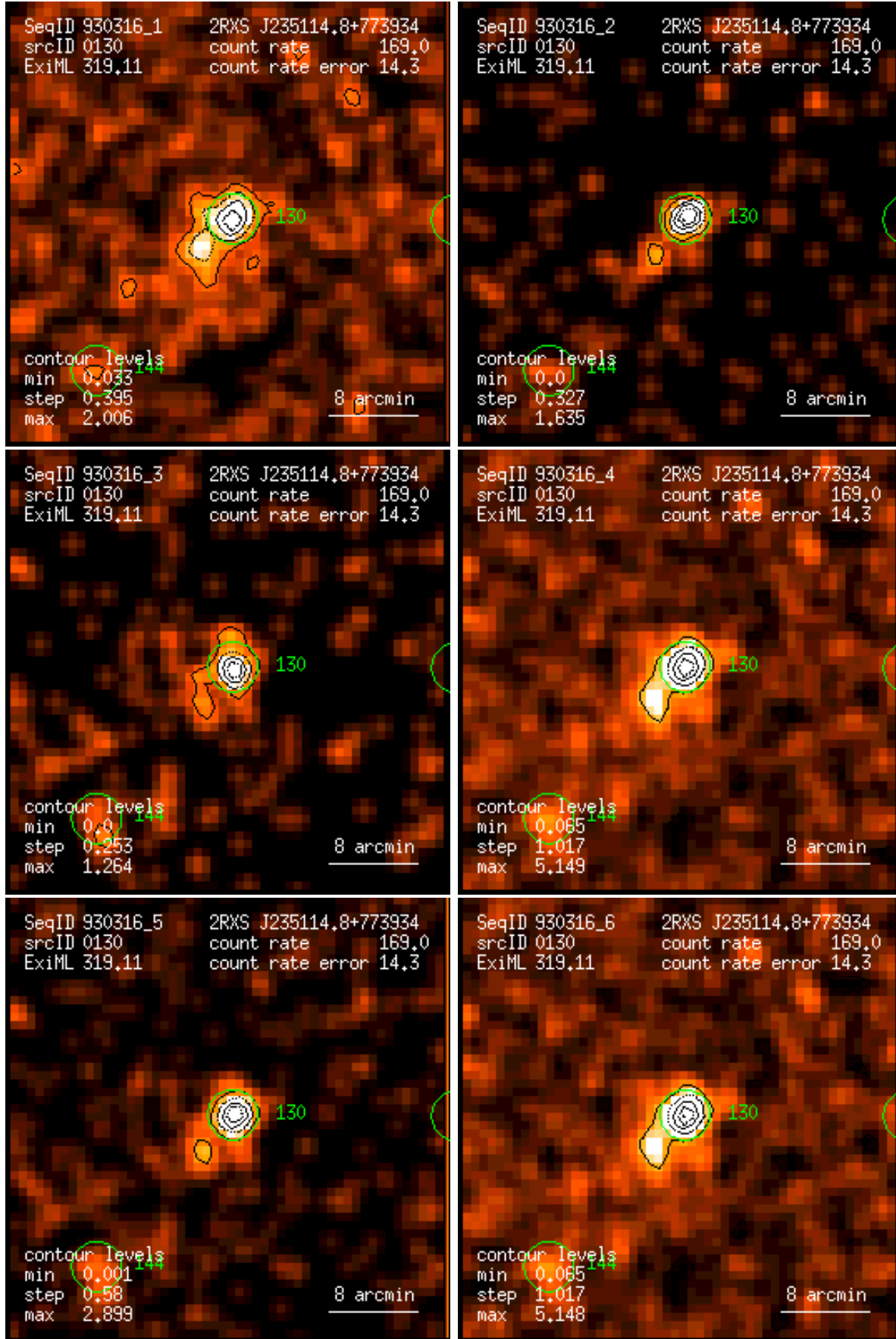
Figure 130: RASS 930316: detection 0130: band rate images, Gaussian filter: (1) PSPC channels 11 – 41, (2) 52 – 90, (3) 91 – 201, (4) 11 – 235, (5) 52 – 201, (6) 11 – 201. Broad band rates in counts/ks. Band rate contour levels in counts/ks/arcmin 2 .
