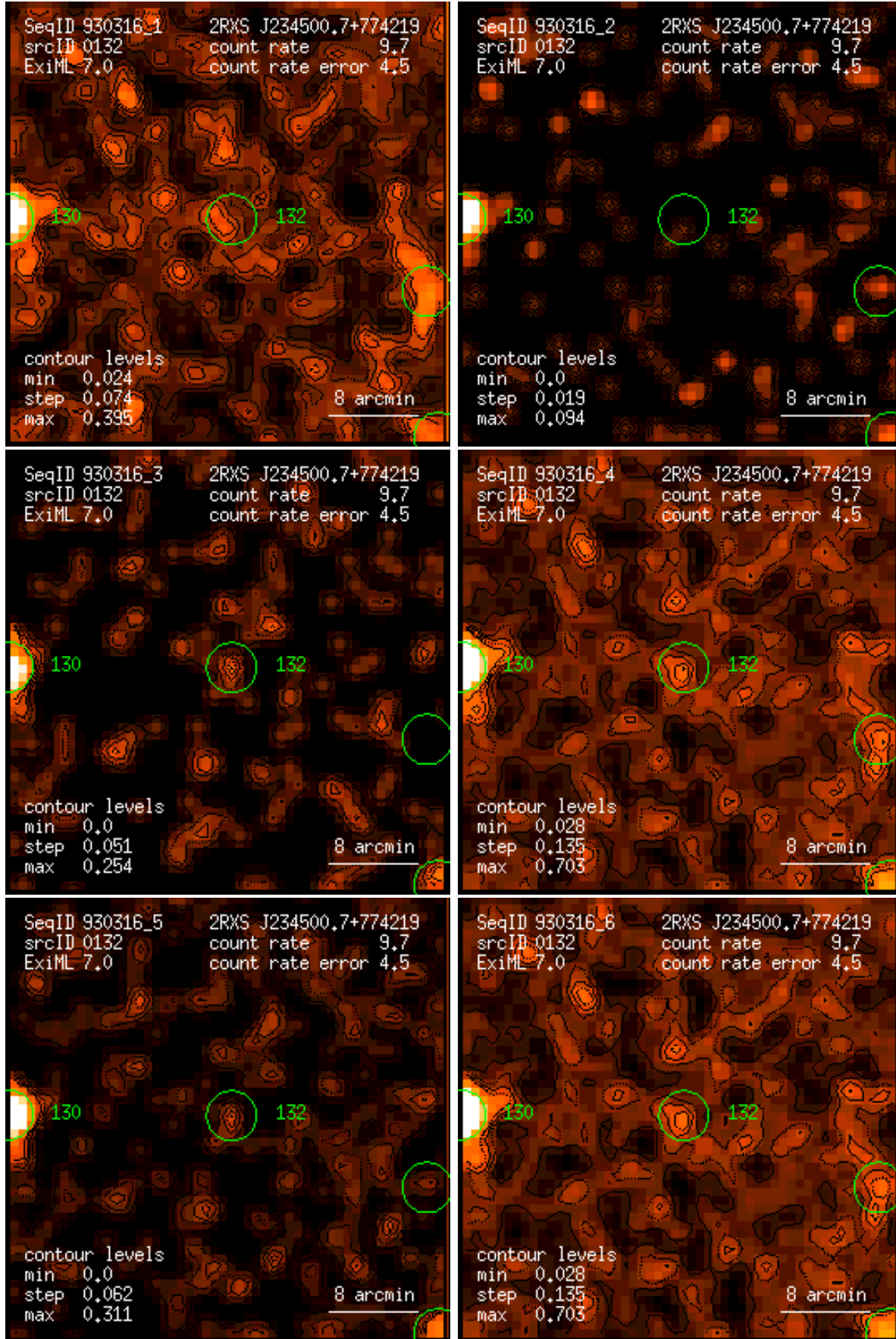
Figure 132: RASS 930316: detection 0132: band rate images, Gaussian filter: (1) PSPC channels 11 – 41, (2) 52 – 90, (3) 91 – 201, (4) 11 – 235, (5) 52 – 201, (6) 11 – 201. Broad band rates in counts/ks. Band rate contour levels in counts/ks/arcmin 2 .
