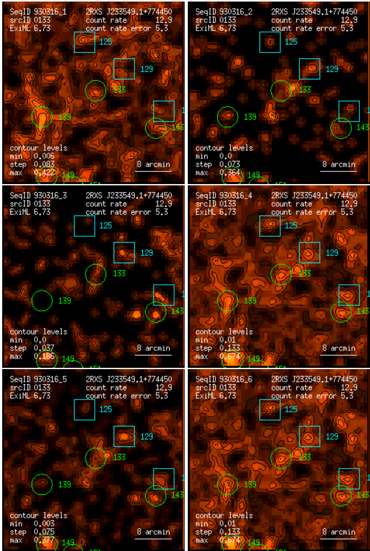
Figure 133: RASS 930316: detection 0133: band rate images, Gaussian filter: (1) PSPC channels 11 – 41, (2) 52 – 90, (3) 91 – 201, (4) 11 – 235, (5) 52 – 201, (6) 11 – 201. Broad band rates in counts/ks. Band rate contour levels in counts/ks/arcmin 2 .
