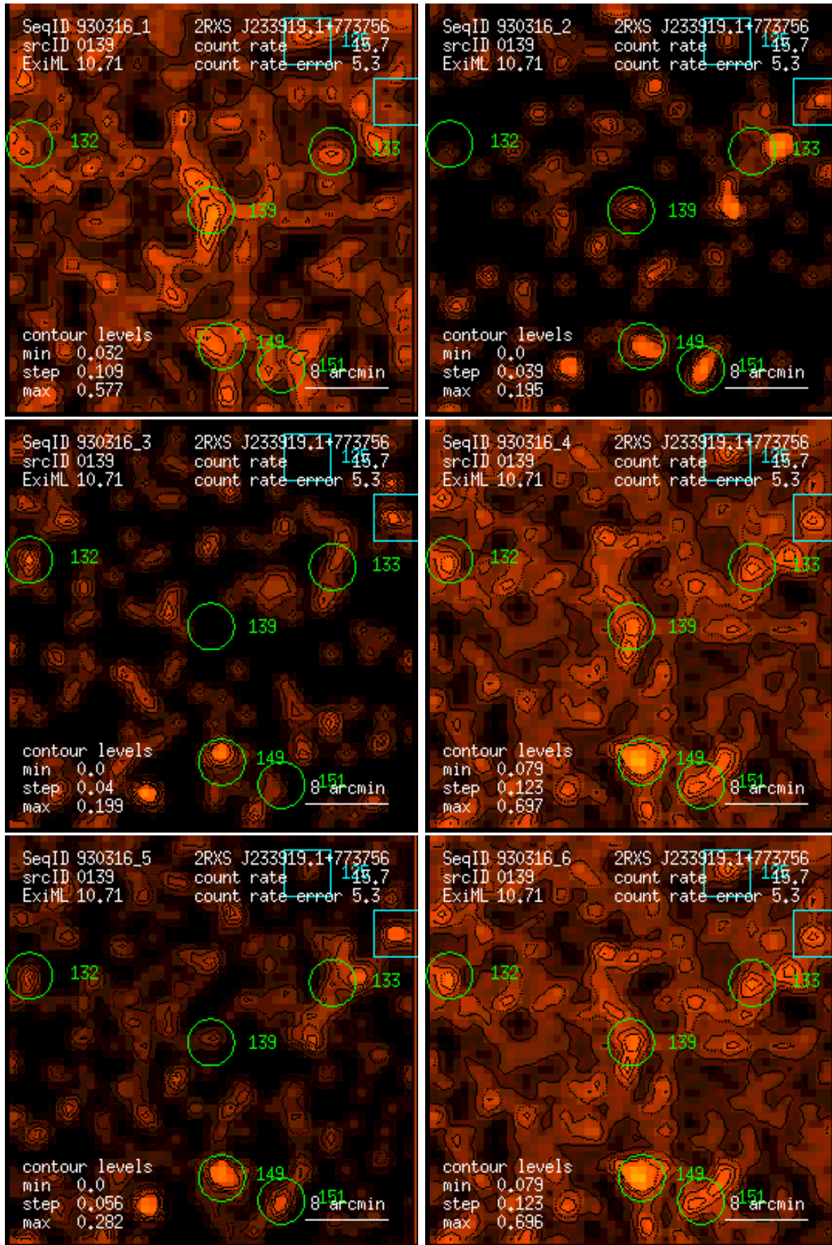
Figure 139: RASS 930316: detection 0139: band rate images, Gaussian filter: (1) PSPC channels 11 – 41, (2) 52 – 90, (3) 91 – 201, (4) 11 – 235, (5) 52 – 201, (6) 11 – 201. Broad band rates in counts/ks. Band rate contour levels in counts/ks/arcmin 2 .
