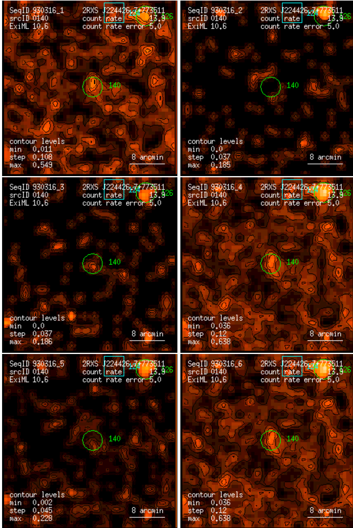
Figure 140: RASS 930316: detection 0140: band rate images, Gaussian filter: (1) PSPC channels 11 – 41, (2) 52 – 90, (3) 91 – 201, (4) 11 – 235, (5) 52 – 201, (6) 11 – 201. Broad band rates in counts/ks. Band rate contour levels in counts/ks/arcmin 2 .
