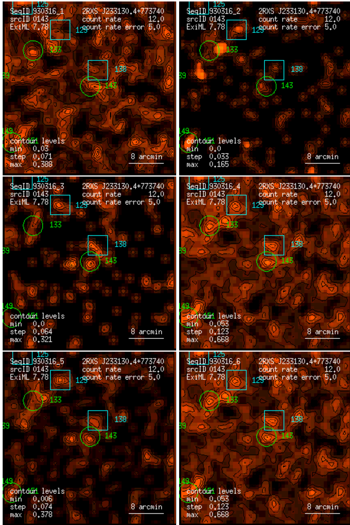
Figure 143: RASS 930316: detection 0143: band rate images, Gaussian filter: (1) PSPC channels 11 – 41, (2) 52 – 90, (3) 91 – 201, (4) 11 – 235, (5) 52 – 201, (6) 11 – 201. Broad band rates in counts/ks. Band rate contour levels in counts/ks/arcmin 2 .
