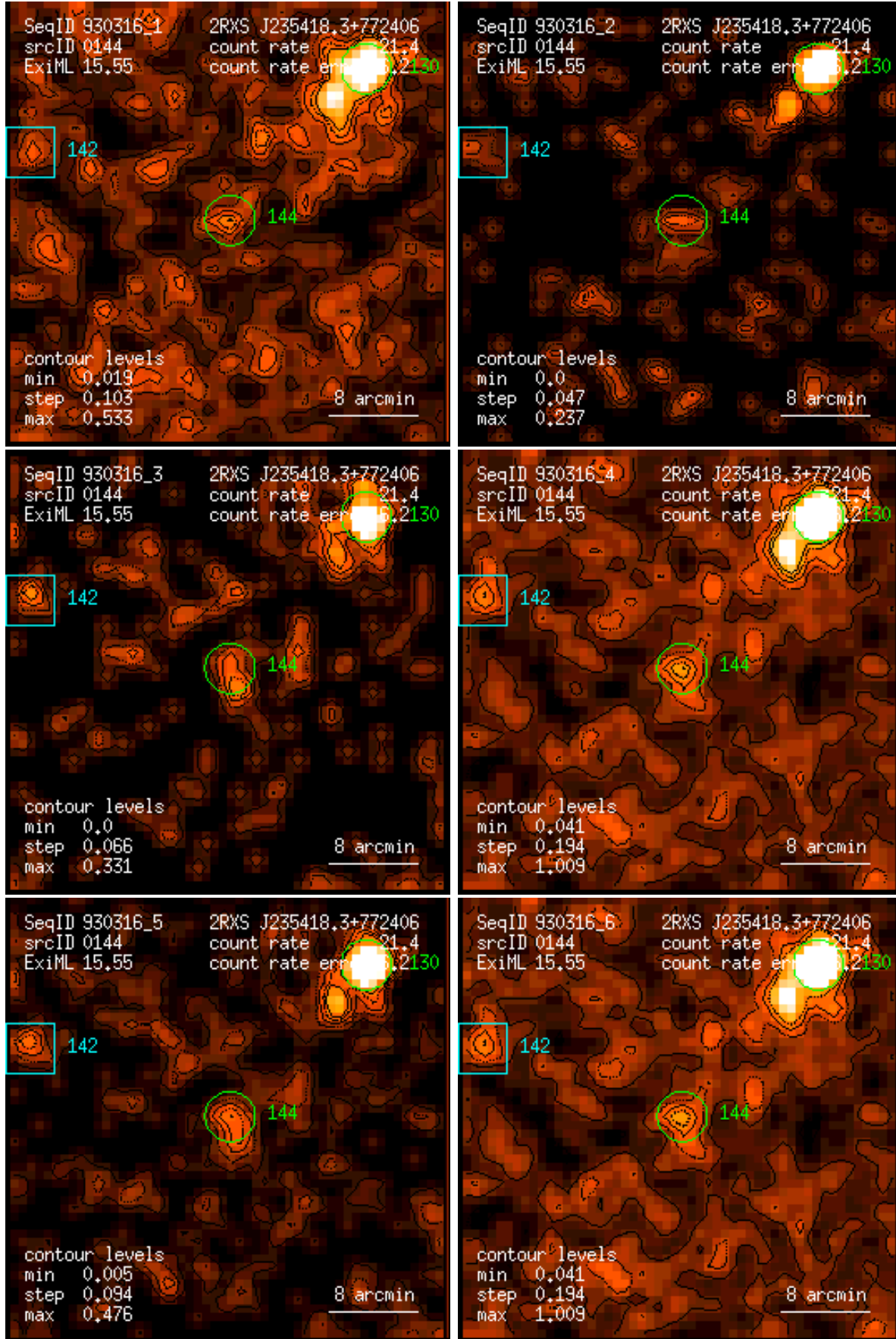
Figure 144: RASS 930316: detection 0144: band rate images, Gaussian filter: (1) PSPC channels 11 – 41, (2) 52 – 90, (3) 91 – 201, (4) 11 – 235, (5) 52 – 201, (6) 11 – 201. Broad band rates in counts/ks. Band rate contour levels in counts/ks/arcmin 2 .
