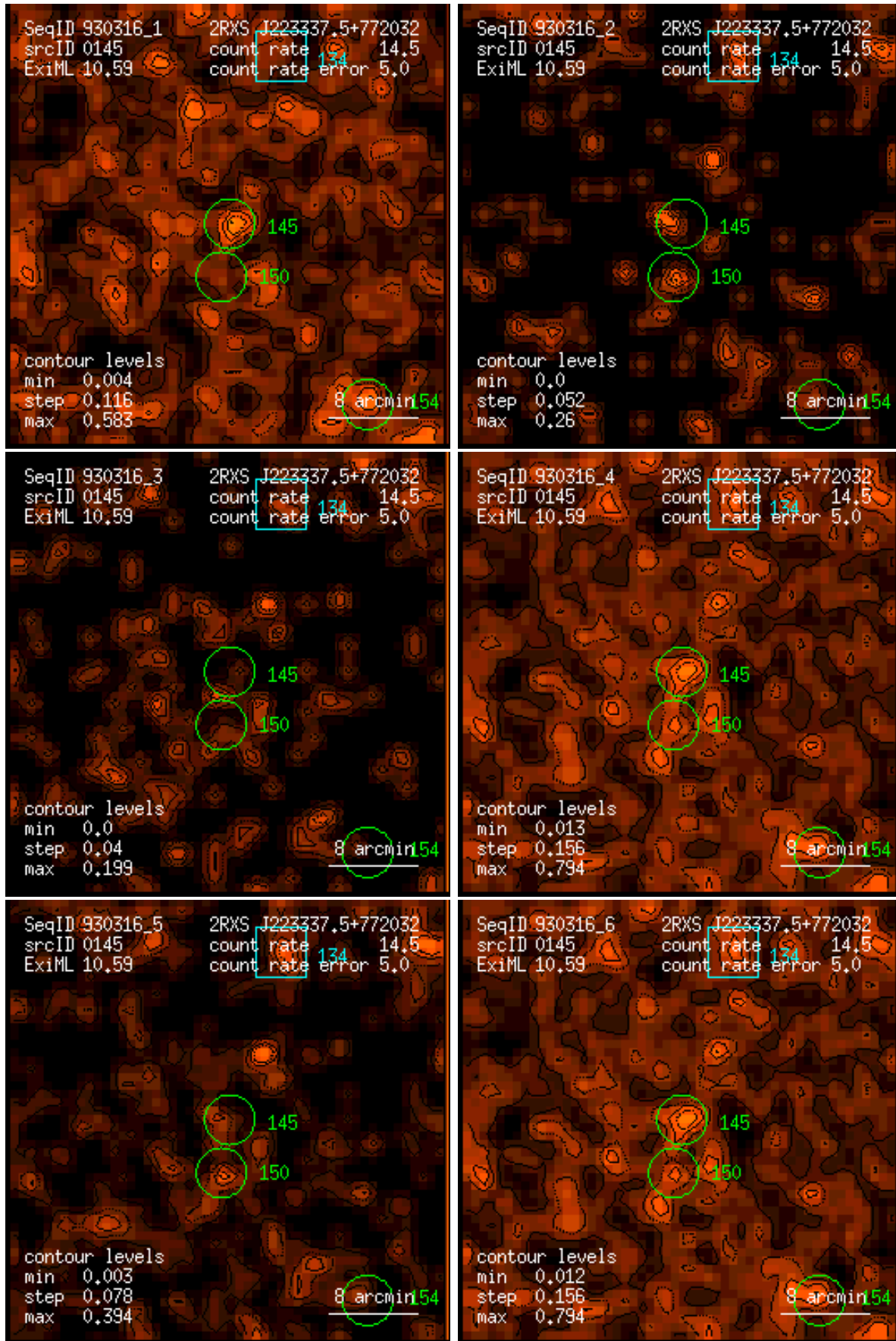
Figure 145: RASS 930316: detection 0145: band rate images, Gaussian filter: (1) PSPC channels 11 – 41, (2) 52 – 90, (3) 91 – 201, (4) 11 – 235, (5) 52 – 201, (6) 11 – 201. Broad band rates in counts/ks. Band rate contour levels in counts/ks/arcmin 2 .
