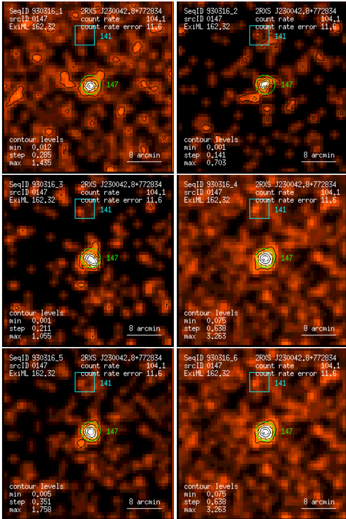
Figure 147: RASS 930316: detection 0147: band rate images, Gaussian filter: (1) PSPC channels 11 – 41, (2) 52 – 90, (3) 91 – 201, (4) 11 – 235, (5) 52 – 201, (6) 11 – 201. Broad band rates in counts/ks. Band rate contour levels in counts/ks/arcmin 2 .
