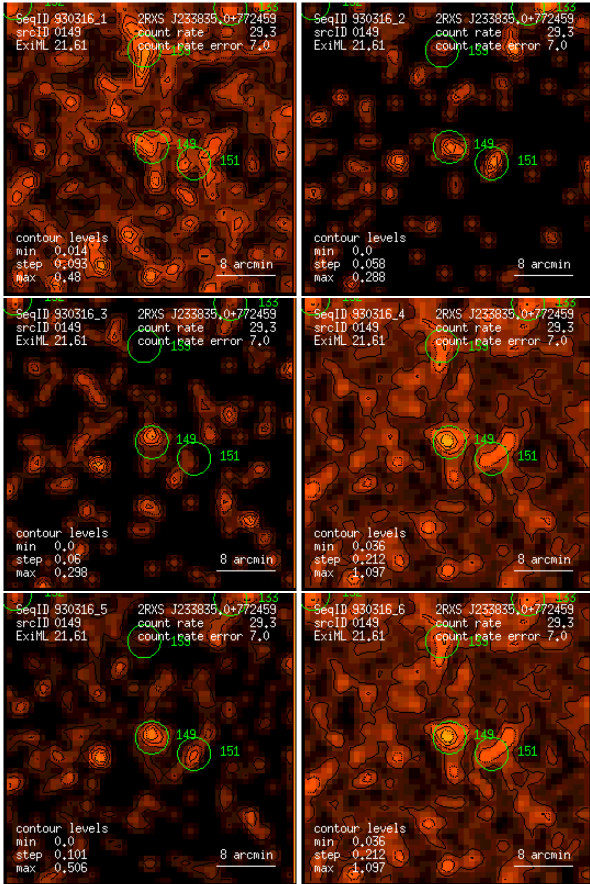
Figure 149: RASS 930316: detection 0149: band rate images, Gaussian filter: (1) PSPC channels 11 – 41, (2) 52 – 90, (3) 91 – 201, (4) 11 – 235, (5) 52 – 201, (6) 11 – 201. Broad band rates in counts/ks. Band rate contour levels in counts/ks/arcmin 2 .
