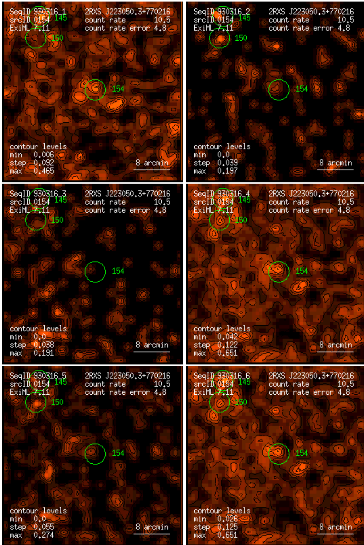
Figure 154: RASS 930316: detection 0154: band rate images, Gaussian filter: (1) PSPC channels 11 – 41, (2) 52 – 90, (3) 91 – 201, (4) 11 – 235, (5) 52 – 201, (6) 11 – 201. Broad band rates in counts/ks. Band rate contour levels in counts/ks/arcmin 2 .
