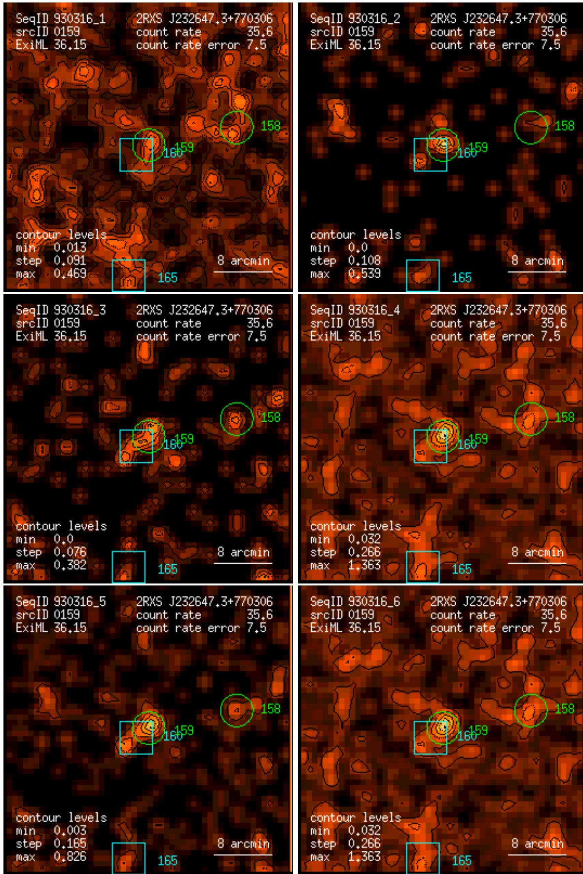
Figure 159: RASS 930316: detection 0159: band rate images, Gaussian filter: (1) PSPC channels 11 – 41, (2) 52 – 90, (3) 91 – 201, (4) 11 – 235, (5) 52 – 201, (6) 11 – 201. Broad band rates in counts/ks. Band rate contour levels in counts/ks/arcmin 2 .
