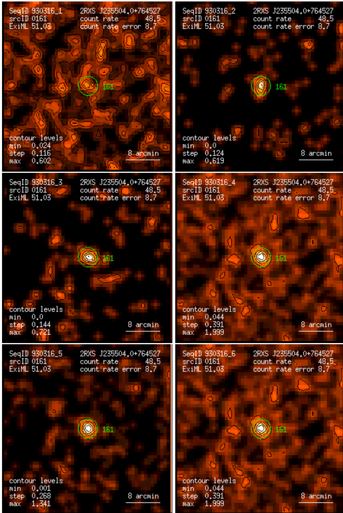
Figure 161: RASS 930316: detection 0161: band rate images, Gaussian filter: (1) PSPC channels 11 – 41, (2) 52 – 90, (3) 91 – 201, (4) 11 – 235, (5) 52 – 201, (6) 11 – 201. Broad band rates in counts/ks. Band rate contour levels in counts/ks/arcmin 2 .
