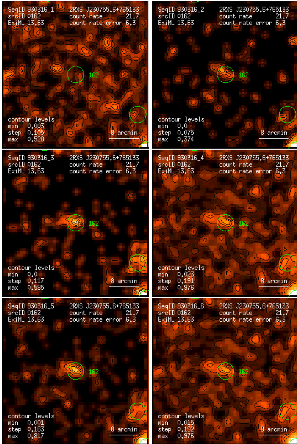
Figure 162: RASS 930316: detection 0162: band rate images, Gaussian filter: (1) PSPC channels 11 – 41, (2) 52 – 90, (3) 91 – 201, (4) 11 – 235, (5) 52 – 201, (6) 11 – 201. Broad band rates in counts/ks. Band rate contour levels in counts/ks/arcmin 2 .
