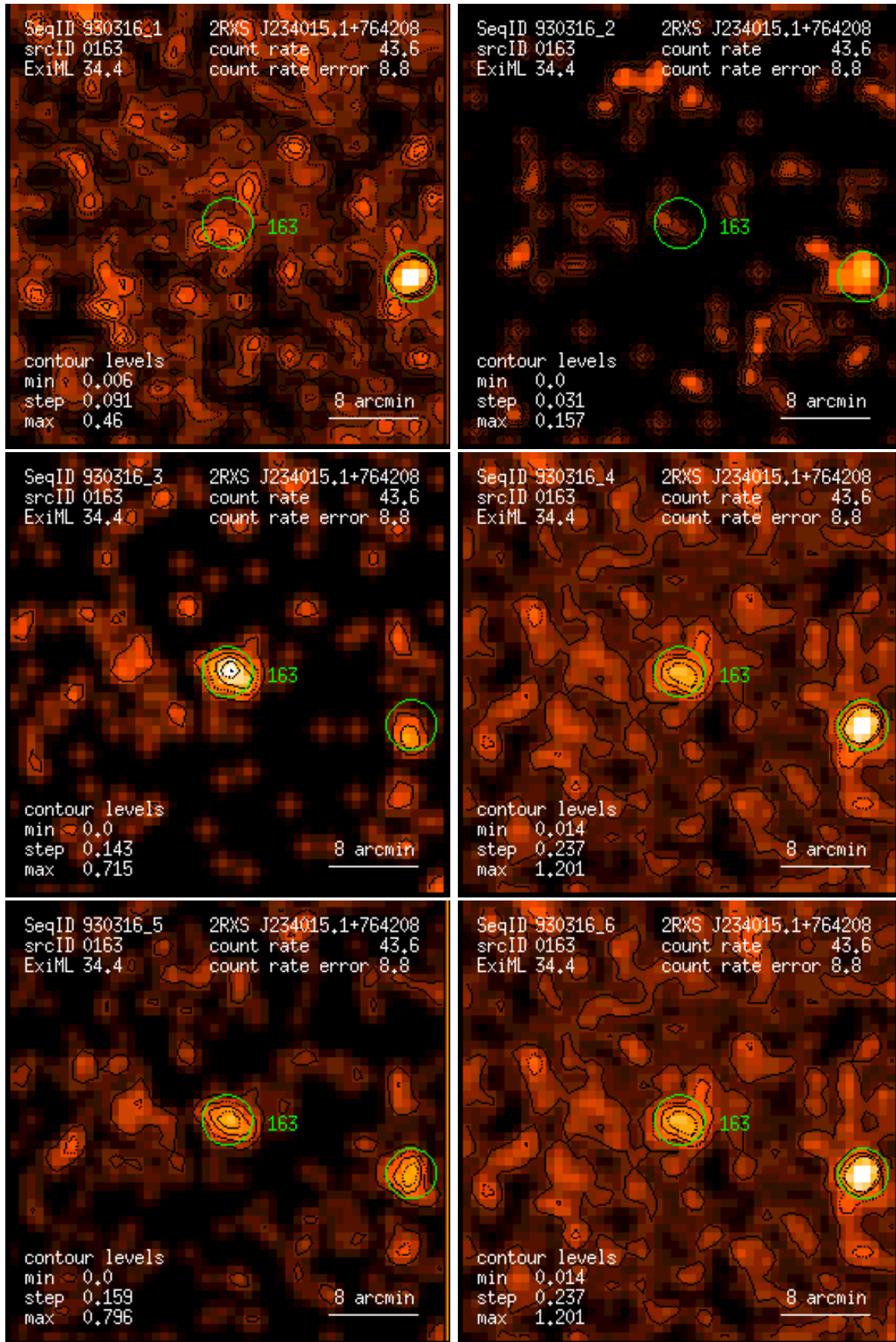
Figure 163: RASS 930316: detection 0163: band rate images, Gaussian filter: (1) PSPC channels 11 – 41, (2) 52 – 90, (3) 91 – 201, (4) 11 – 235, (5) 52 – 201, (6) 11 – 201. Broad band rates in counts/ks. Band rate contour levels in counts/ks/arcmin 2 .
