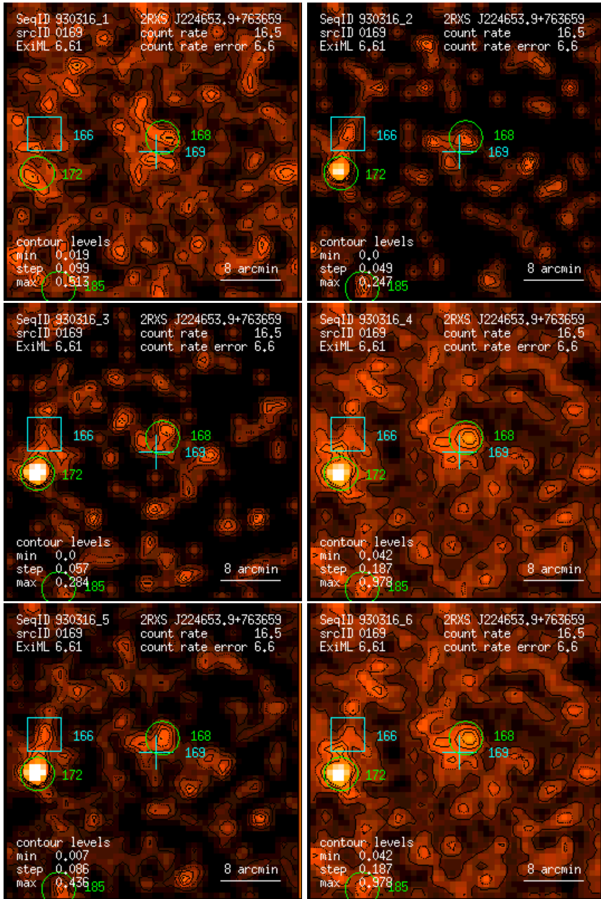
Figure 169: RASS 930316: detection 0169: band rate images, Gaussian filter: (1) PSPC channels 11 – 41, (2) 52 – 90, (3) 91 – 201, (4) 11 – 235, (5) 52 – 201, (6) 11 – 201. Broad band rates in counts/ks. Band rate contour levels in counts/ks/arcmin 2 .
