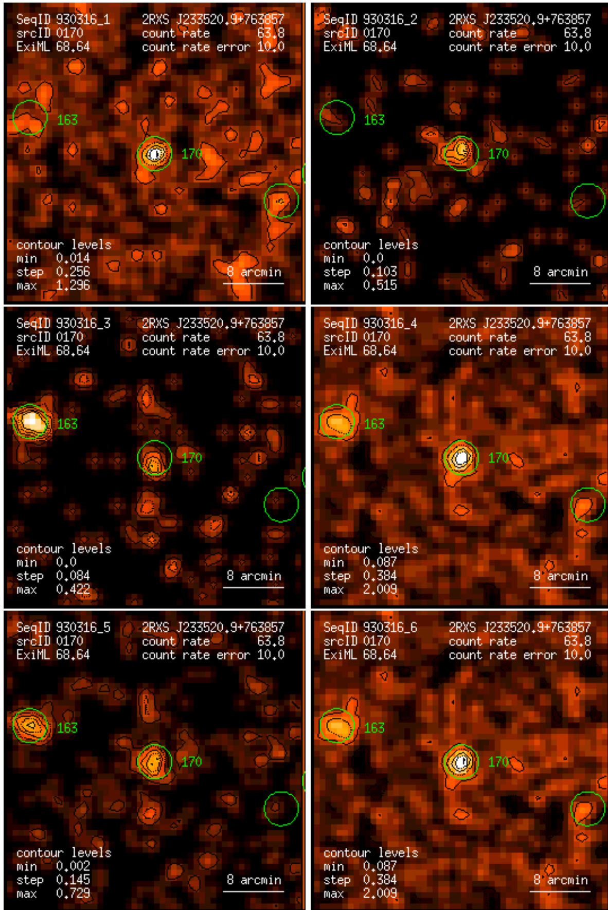
Figure 170: RASS 930316: detection 0170: band rate images, Gaussian filter: (1) PSPC channels 11 – 41, (2) 52 – 90, (3) 91 – 201, (4) 11 – 235, (5) 52 – 201, (6) 11 – 201. Broad band rates in counts/ks. Band rate contour levels in counts/ks/arcmin 2 .
