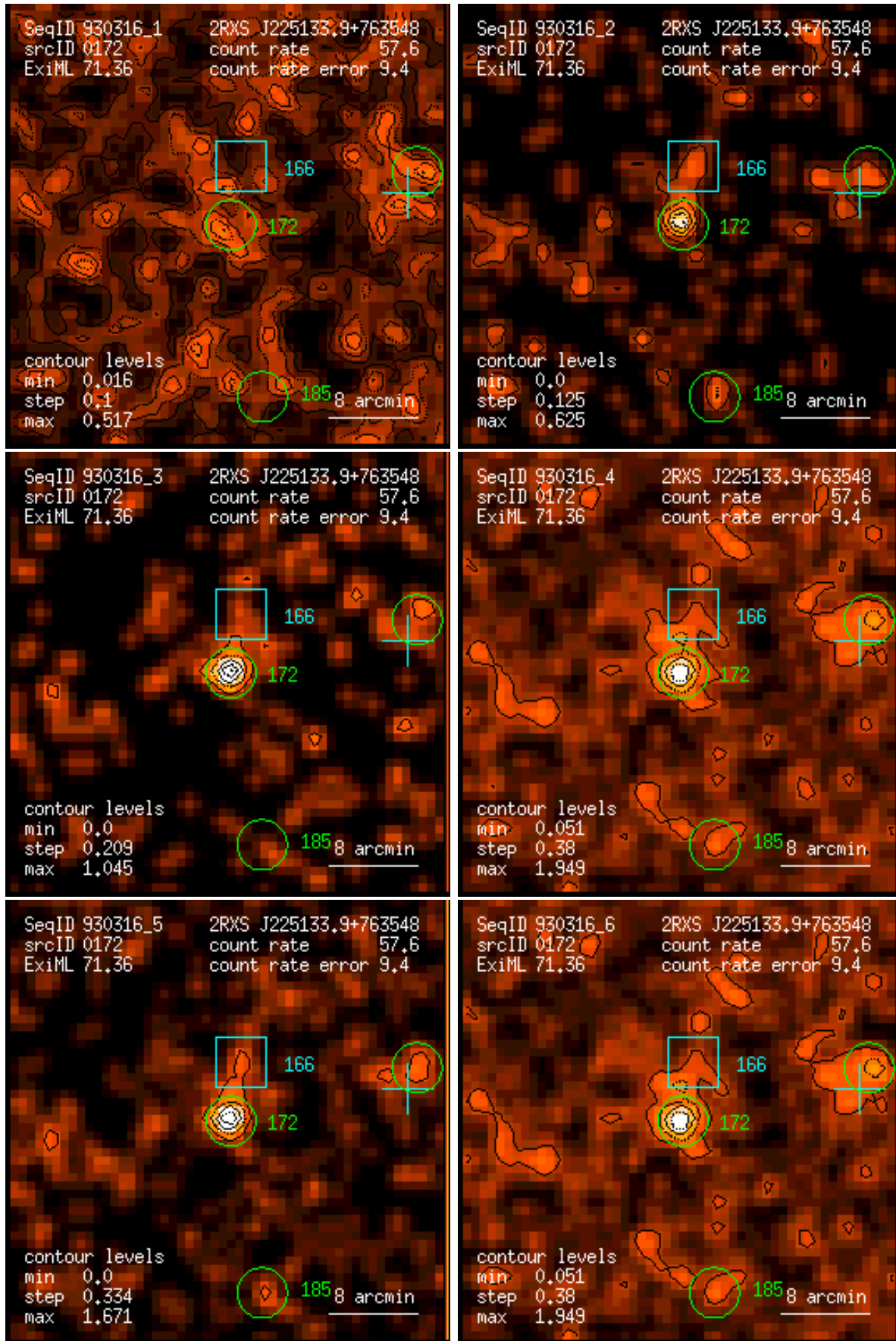
Figure 172: RASS 930316: detection 0172: band rate images, Gaussian filter: (1) PSPC channels 11 – 41, (2) 52 – 90, (3) 91 – 201, (4) 11 – 235, (5) 52 – 201, (6) 11 – 201. Broad band rates in counts/ks. Band rate contour levels in counts/ks/arcmin 2 .
