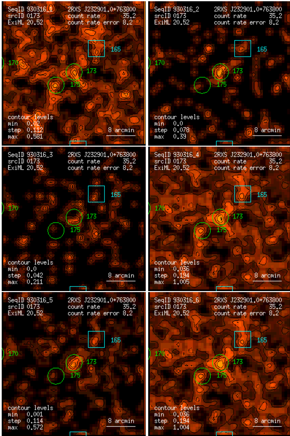
Figure 173: RASS 930316: detection 0173: band rate images, Gaussian filter: (1) PSPC channels 11 – 41, (2) 52 – 90, (3) 91 – 201, (4) 11 – 235, (5) 52 – 201, (6) 11 – 201. Broad band rates in counts/ks. Band rate contour levels in counts/ks/arcmin 2 .
