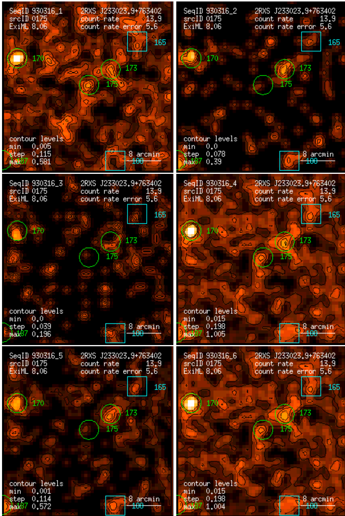
Figure 175: RASS 930316: detection 0175: band rate images, Gaussian filter: (1) PSPC channels 11 – 41, (2) 52 – 90, (3) 91 – 201, (4) 11 – 235, (5) 52 – 201, (6) 11 – 201. Broad band rates in counts/ks. Band rate contour levels in counts/ks/arcmin 2 .
