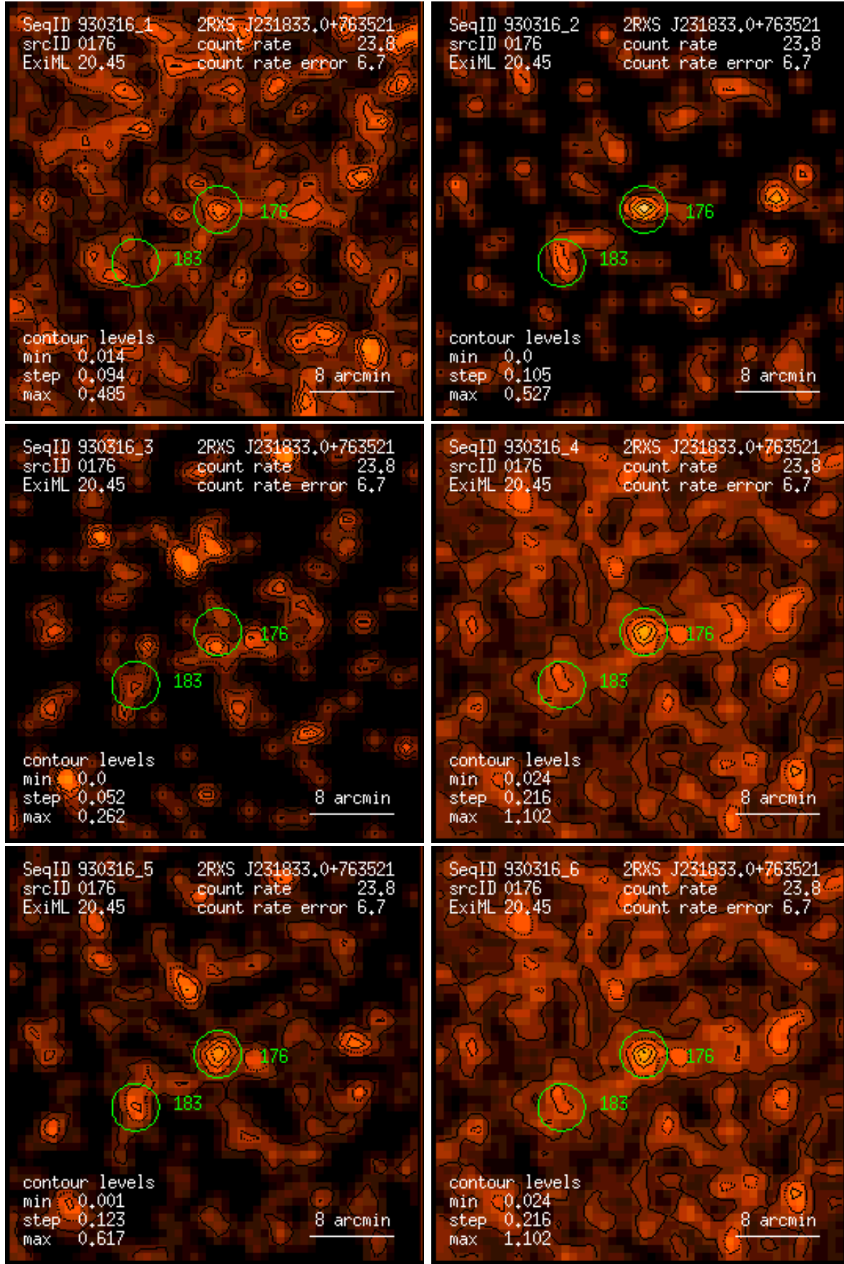
Figure 176: RASS 930316: detection 0176: band rate images, Gaussian filter: (1) PSPC channels 11 – 41, (2) 52 – 90, (3) 91 – 201, (4) 11 – 235, (5) 52 – 201, (6) 11 – 201. Broad band rates in counts/ks. Band rate contour levels in counts/ks/arcmin 2 .
