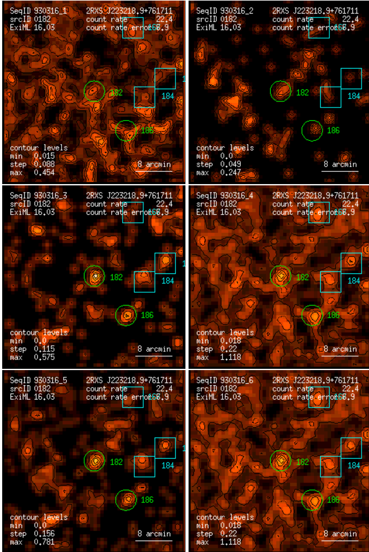
Figure 182: RASS 930316: detection 0182: band rate images, Gaussian filter: (1) PSPC channels 11 – 41, (2) 52 – 90, (3) 91 – 201, (4) 11 – 235, (5) 52 – 201, (6) 11 – 201. Broad band rates in counts/ks. Band rate contour levels in counts/ks/arcmin 2 .
