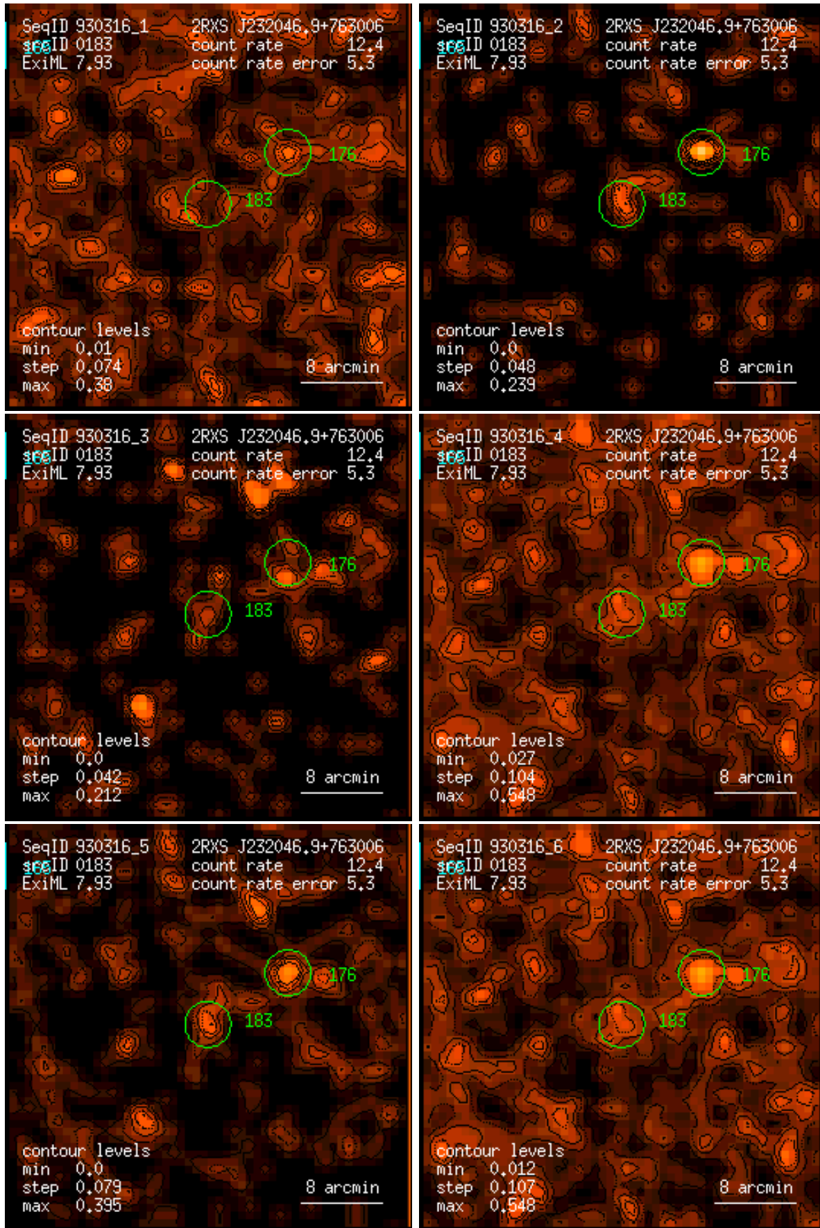
Figure 183: RASS 930316: detection 0183: band rate images, Gaussian filter: (1) PSPC channels 11 – 41, (2) 52 – 90, (3) 91 – 201, (4) 11 – 235, (5) 52 – 201, (6) 11 – 201. Broad band rates in counts/ks. Band rate contour levels in counts/ks/arcmin 2 .
