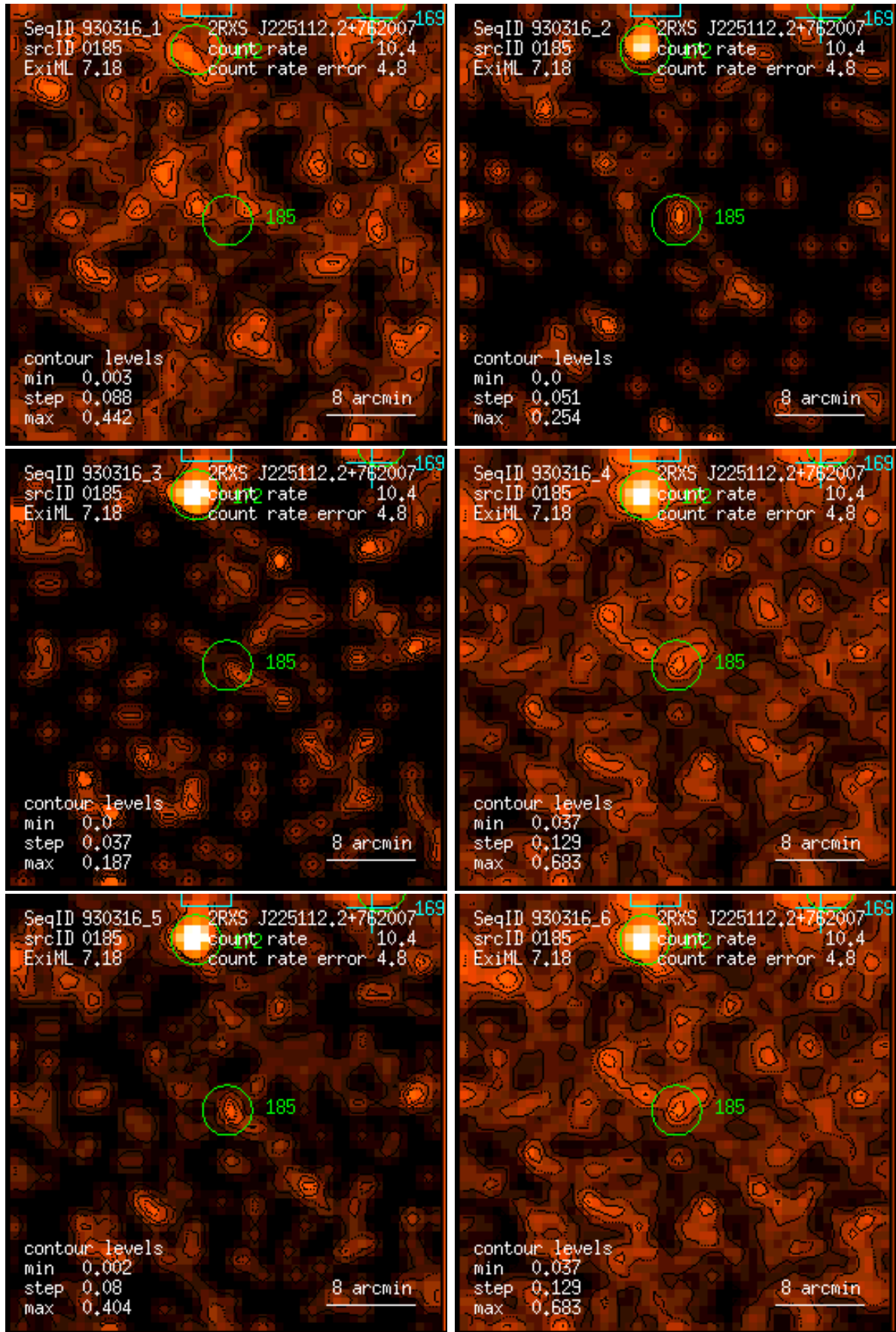
Figure 185: RASS 930316: detection 0185: band rate images, Gaussian filter: (1) PSPC channels 11 – 41, (2) 52 – 90, (3) 91 – 201, (4) 11 – 235, (5) 52 – 201, (6) 11 – 201. Broad band rates in counts/ks. Band rate contour levels in counts/ks/arcmin 2 .
