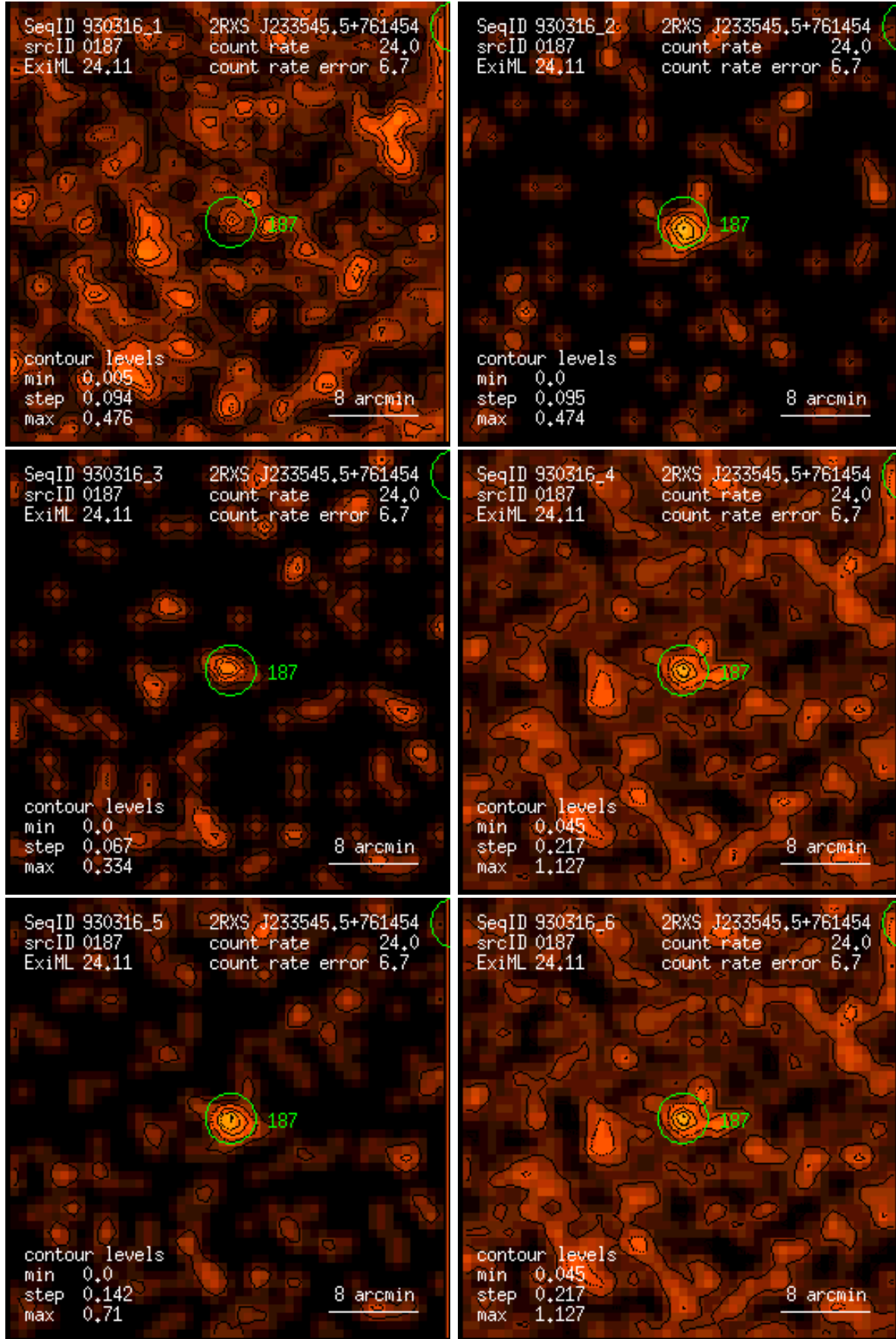
Figure 187: RASS 930316: detection 0187: band rate images, Gaussian filter: (1) PSPC channels 11 – 41, (2) 52 – 90, (3) 91 – 201, (4) 11 – 235, (5) 52 – 201, (6) 11 – 201. Broad band rates in counts/ks. Band rate contour levels in counts/ks/arcmin 2 .
