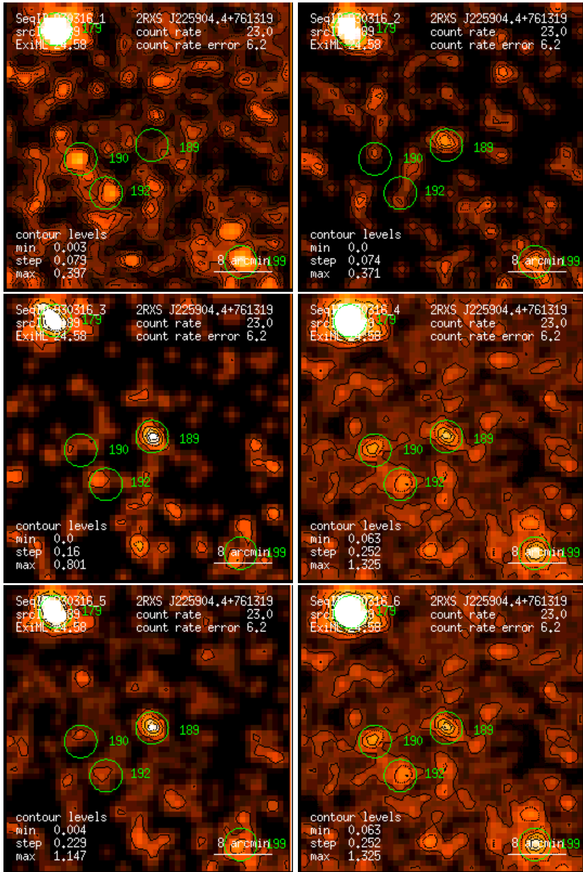
Figure 189: RASS 930316: detection 0189: band rate images, Gaussian filter: (1) PSPC channels 11 – 41, (2) 52 – 90, (3) 91 – 201, (4) 11 – 235, (5) 52 – 201, (6) 11 – 201. Broad band rates in counts/ks. Band rate contour levels in counts/ks/arcmin 2 .
