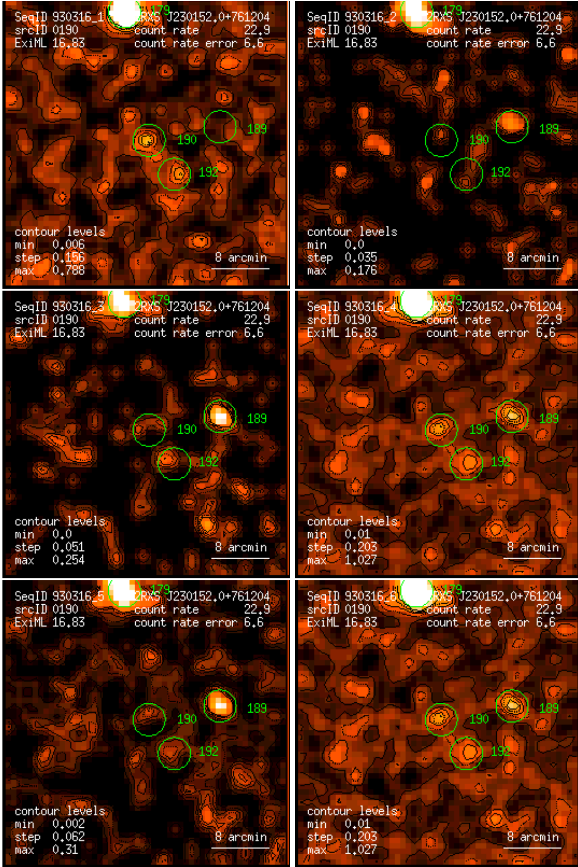
Figure 190: RASS 930316: detection 0190: band rate images, Gaussian filter: (1) PSPC channels 11 – 41, (2) 52 – 90, (3) 91 – 201, (4) 11 – 235, (5) 52 – 201, (6) 11 – 201. Broad band rates in counts/ks. Band rate contour levels in counts/ks/arcmin 2 .
