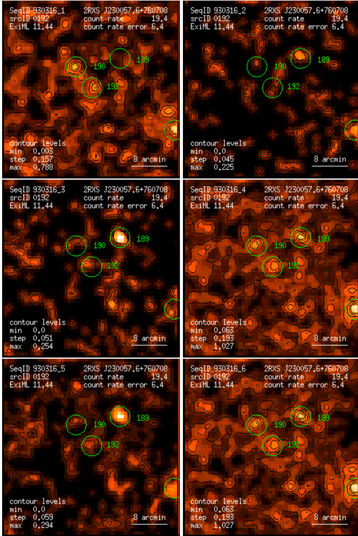
Figure 192: RASS 930316: detection 0192: band rate images, Gaussian filter: (1) PSPC channels 11 – 41, (2) 52 – 90, (3) 91 – 201, (4) 11 – 235, (5) 52 – 201, (6) 11 – 201. Broad band rates in counts/ks. Band rate contour levels in counts/ks/arcmin 2 .
