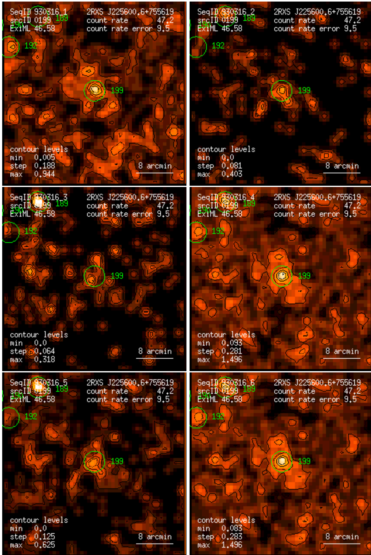
Figure 199: RASS 930316: detection 0199: band rate images, Gaussian filter: (1) PSPC channels 11 – 41, (2) 52 – 90, (3) 91 – 201, (4) 11 – 235, (5) 52 – 201, (6) 11 – 201. Broad band rates in counts/ks. Band rate contour levels in counts/ks/arcmin 2 .
