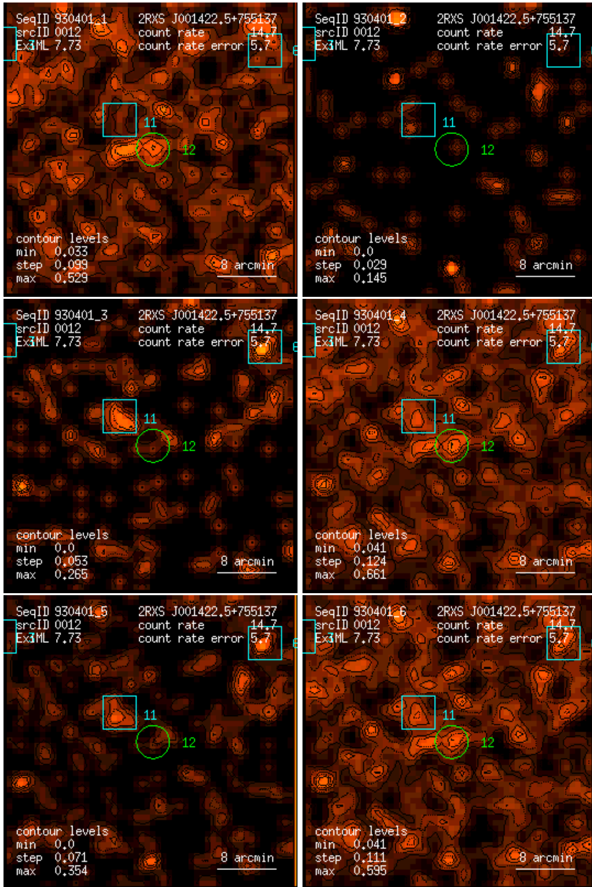
Figure 12: RASS 930401: detection 0012: band rate images, Gaussian filter: (1) PSPC channels 11 – 41, (2) 52 – 90, (3) 91 – 201, (4) 11 – 235, (5) 52 – 201, (6) 11 – 201. Broad band rates in counts/ks. Band rate contour levels in counts/ks/arcmin 2 .
