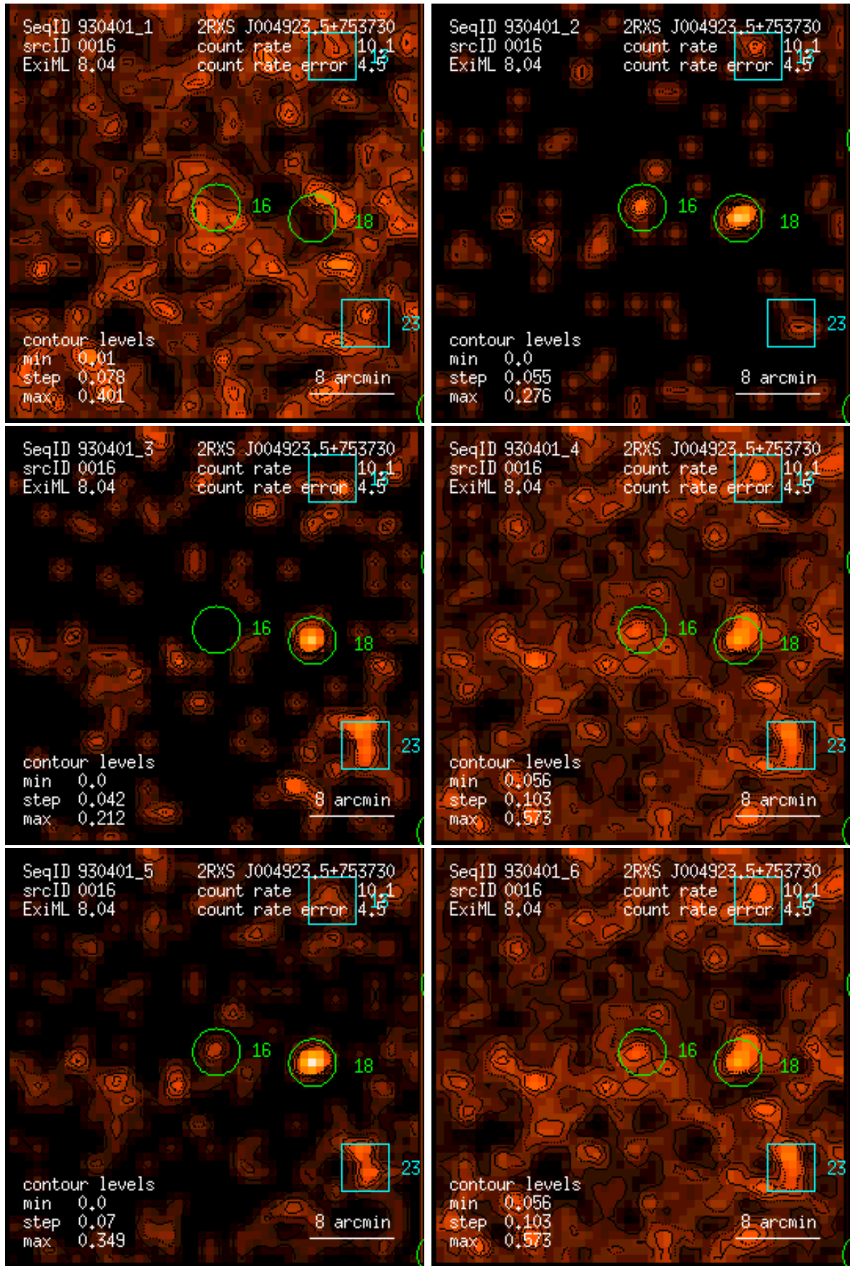
Figure 16: RASS 930401: detection 0016: band rate images, Gaussian filter: (1) PSPC channels 11 – 41, (2) 52 – 90, (3) 91 – 201, (4) 11 – 235, (5) 52 – 201, (6) 11 – 201. Broad band rates in counts/ks. Band rate contour levels in counts/ks/arcmin 2 .
