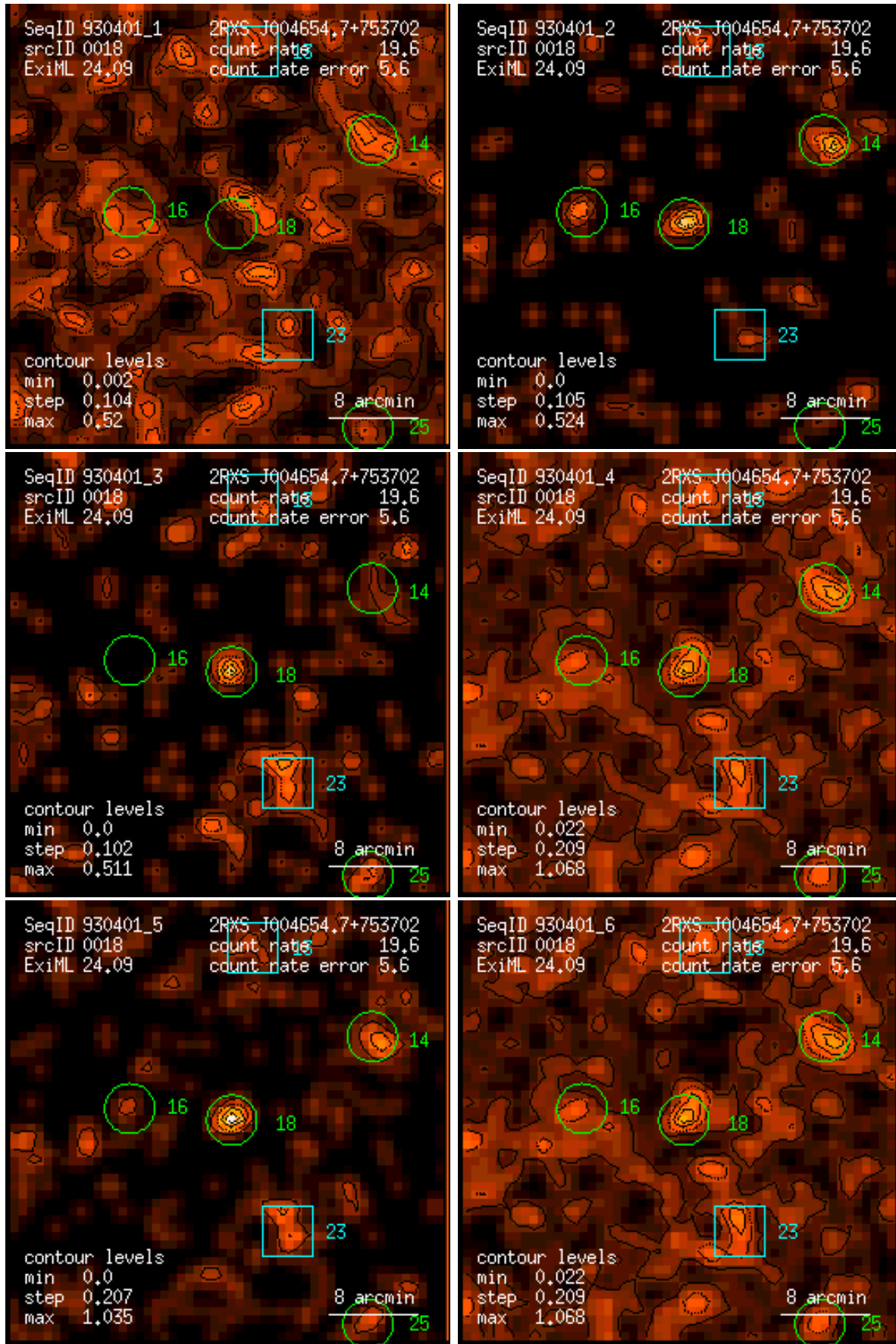
Figure 18: RASS 930401: detection 0018: band rate images, Gaussian filter: (1) PSPC channels 11 – 41, (2) 52 – 90, (3) 91 – 201, (4) 11 – 235, (5) 52 – 201, (6) 11 – 201. Broad band rates in counts/ks. Band rate contour levels in counts/ks/arcmin 2 .
