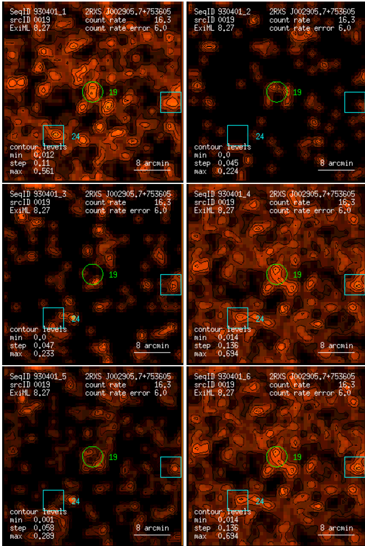
Figure 19: RASS 930401: detection 0019: band rate images, Gaussian filter: (1) PSPC channels 11 – 41, (2) 52 – 90, (3) 91 – 201, (4) 11 – 235, (5) 52 – 201, (6) 11 – 201. Broad band rates in counts/ks. Band rate contour levels in counts/ks/arcmin 2 .
