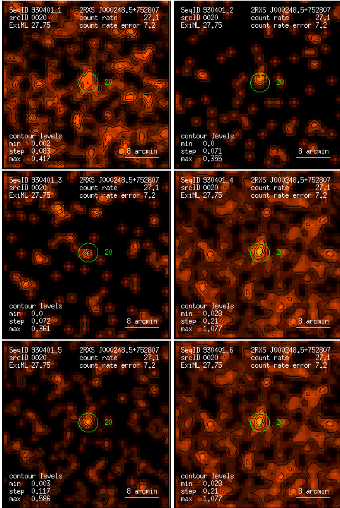
Figure 20: RASS 930401: detection 0020: band rate images, Gaussian filter: (1) PSPC channels 11 – 41, (2) 52 – 90, (3) 91 – 201, (4) 11 – 235, (5) 52 – 201, (6) 11 – 201. Broad band rates in counts/ks. Band rate contour levels in counts/ks/arcmin 2 .
