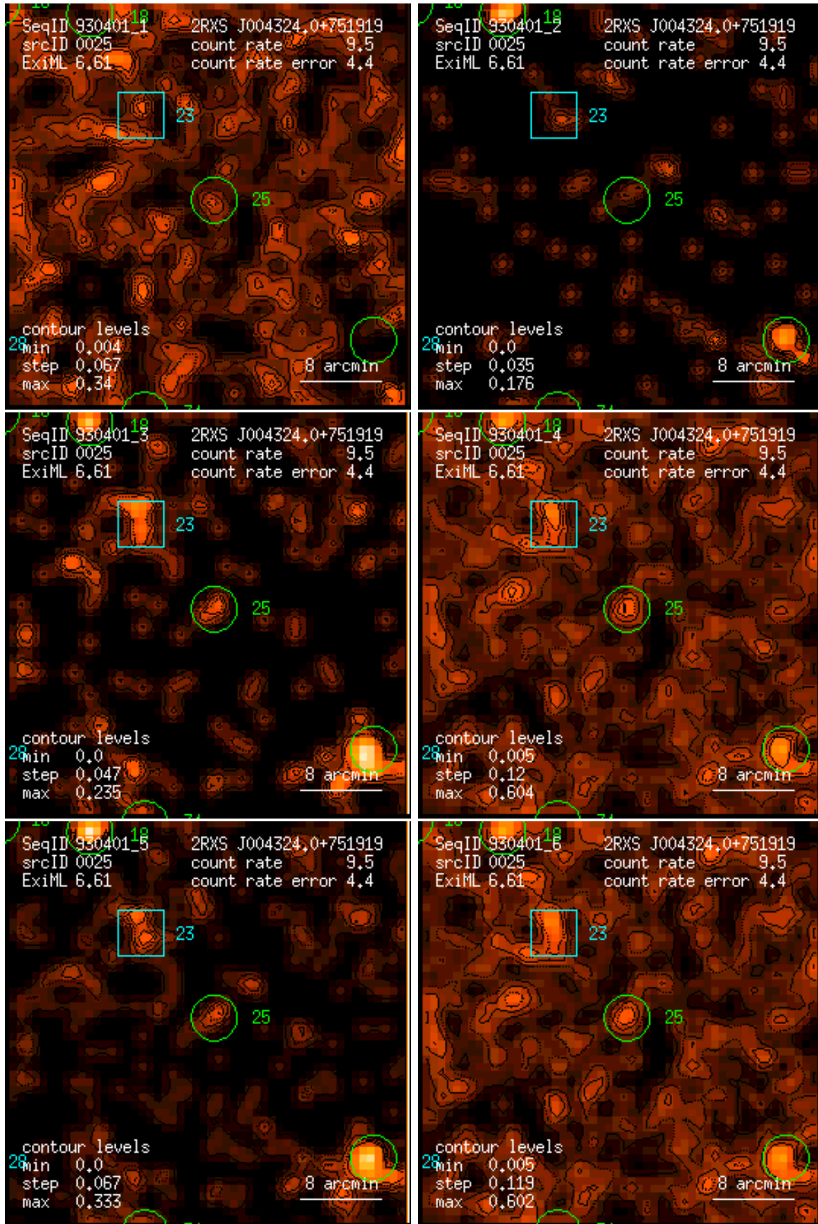
Figure 25: RASS 930401: detection 0025: band rate images, Gaussian filter: (1) PSPC channels 11 – 41, (2) 52 – 90, (3) 91 – 201, (4) 11 – 235, (5) 52 – 201, (6) 11 – 201. Broad band rates in counts/ks. Band rate contour levels in counts/ks/arcmin 2 .
