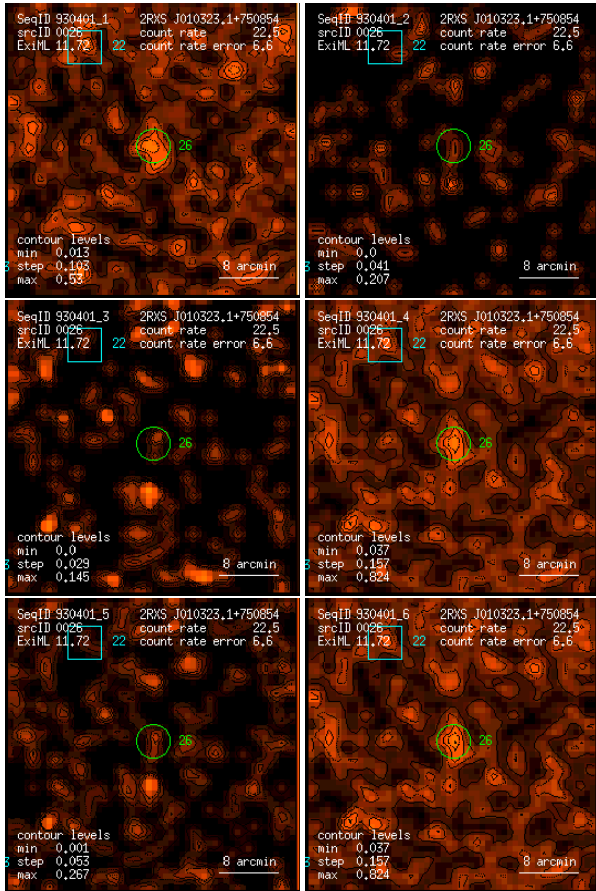
Figure 26: RASS 930401: detection 0026: band rate images, Gaussian filter: (1) PSPC channels 11 – 41, (2) 52 – 90, (3) 91 – 201, (4) 11 – 235, (5) 52 – 201, (6) 11 – 201. Broad band rates in counts/ks. Band rate contour levels in counts/ks/arcmin 2 .
