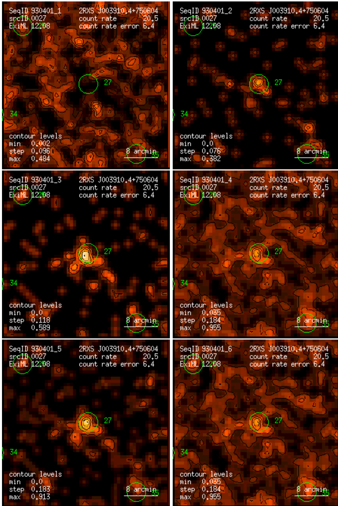
Figure 27: RASS 930401: detection 0027: band rate images, Gaussian filter: (1) PSPC channels 11 – 41, (2) 52 – 90, (3) 91 – 201, (4) 11 – 235, (5) 52 – 201, (6) 11 – 201. Broad band rates in counts/ks. Band rate contour levels in counts/ks/arcmin 2 .
