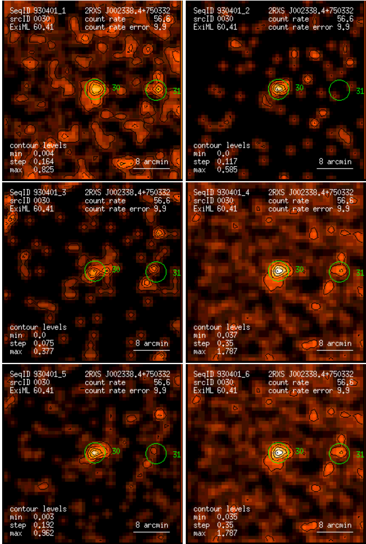
Figure 30: RASS 930401: detection 0030: band rate images, Gaussian filter: (1) PSPC channels 11 – 41, (2) 52 – 90, (3) 91 – 201, (4) 11 – 235, (5) 52 – 201, (6) 11 – 201. Broad band rates in counts/ks. Band rate contour levels in counts/ks/arcmin 2 .
